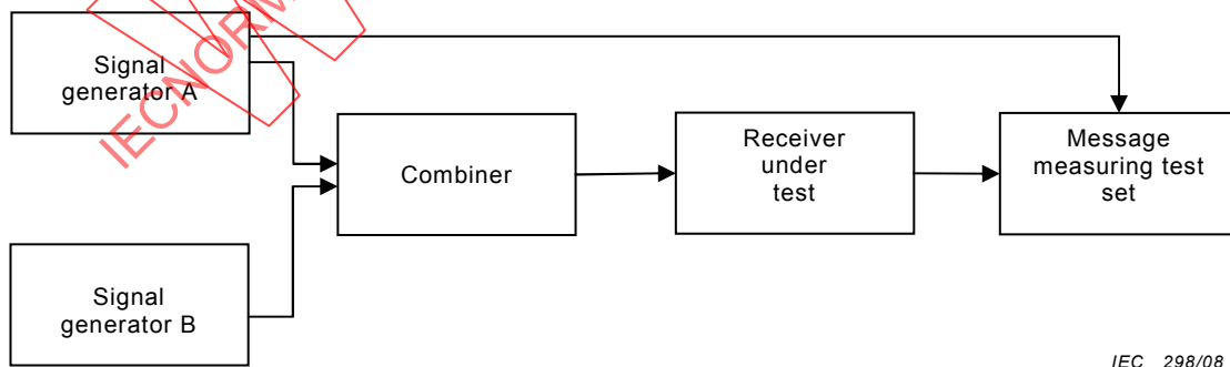
Figure 15 – Measurement arrangement
