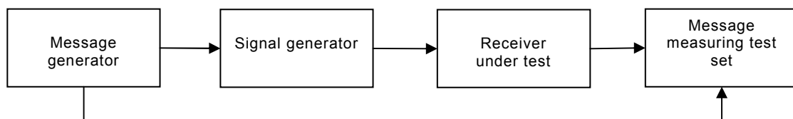
Figure 13 – Measurement arrangement
