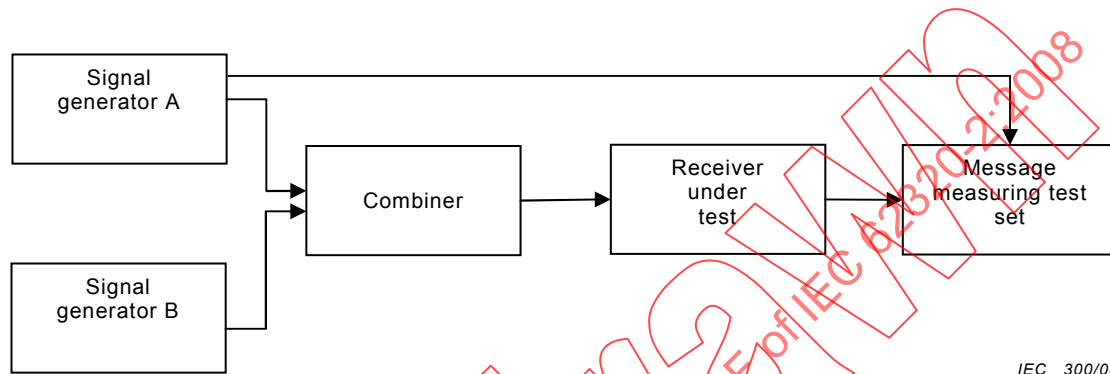
Figure 17 – PER/BER or SINAD measuring equipment
