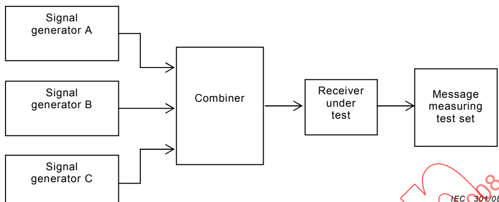
Figure 18 – Measurement arrangement for inter-modulation
