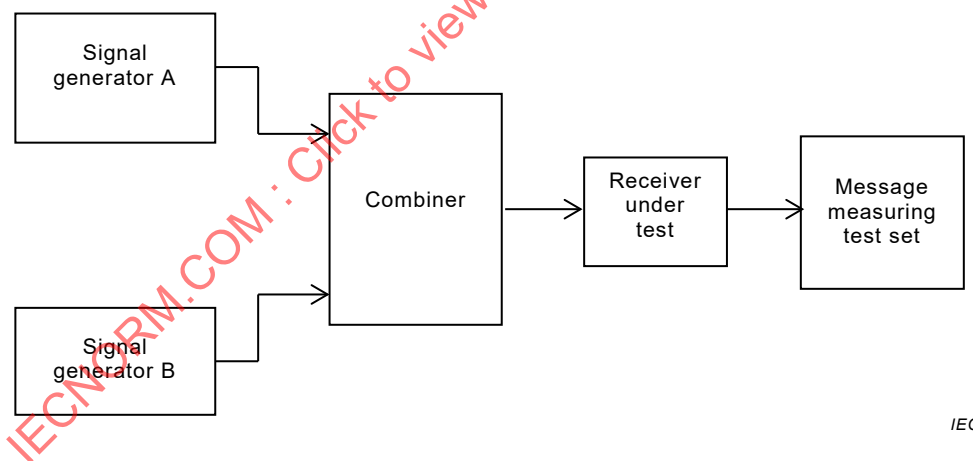
Figure 19 – Measurement arrangement for blocking or desensitisation
