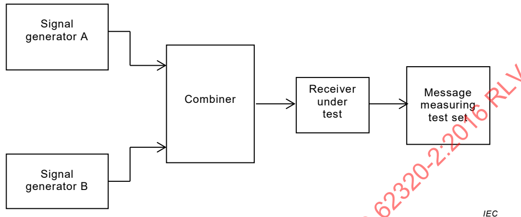
Figure 19 – Measurement arrangement for blocking or desensitisation
