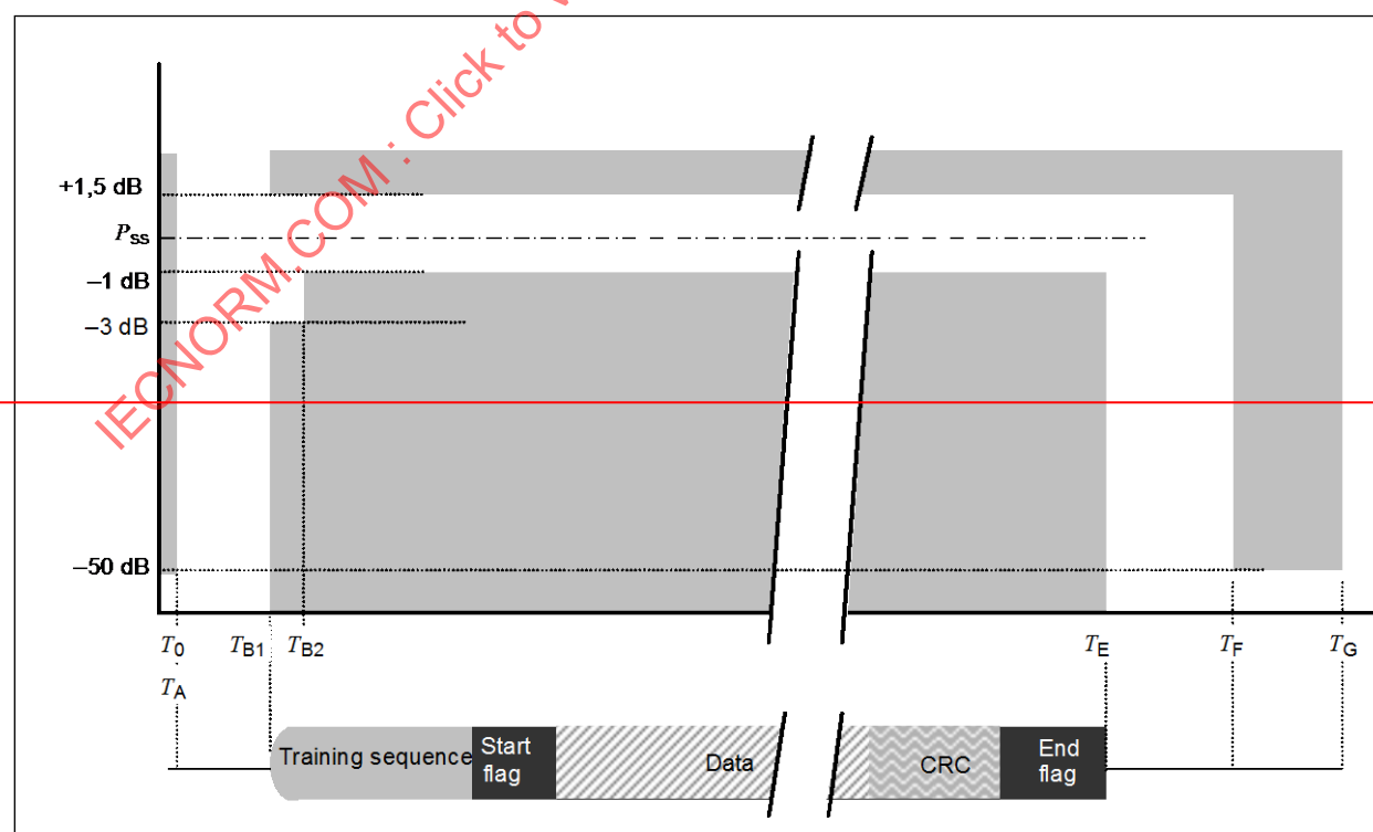
Figure 12 – Power versus time mask
