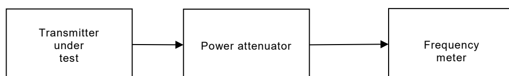
Figure 9 – Measurement arrangement for frequency error
