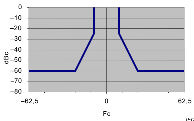
Figure 11 – Emission mask
