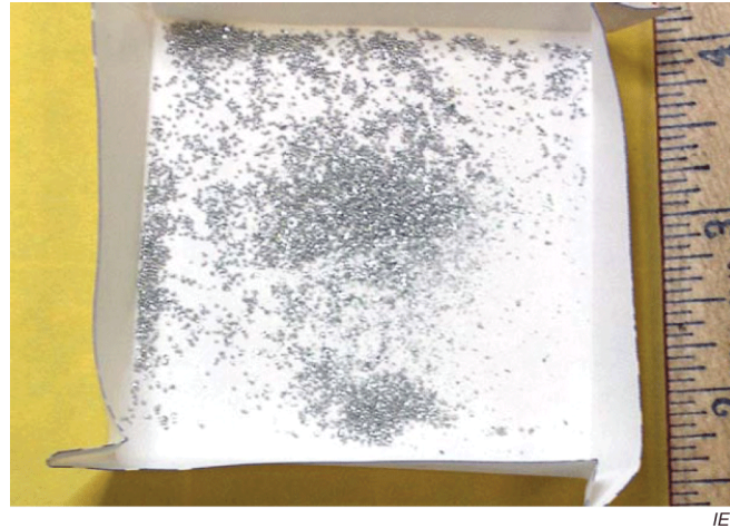
Figure E.12 – Solder ball material collected from BGA using hand removal procedure
