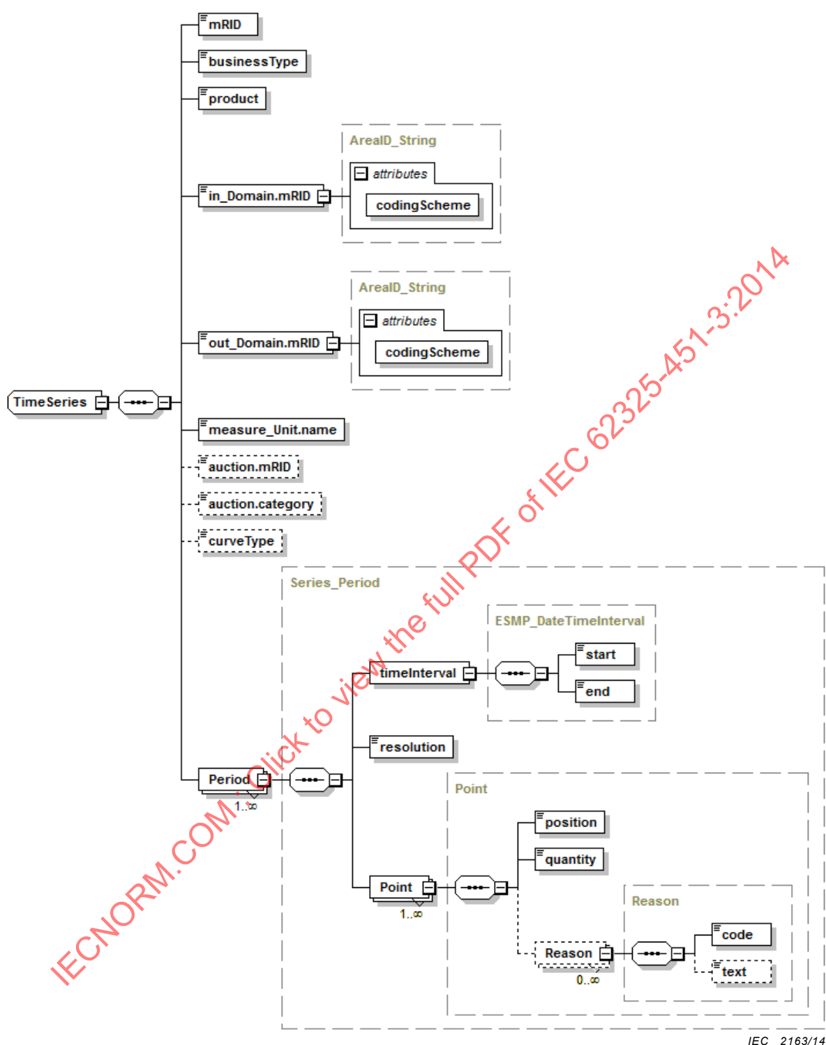
Figure 30 – Capacity_MarketDocument XML schema structure – 2/2
