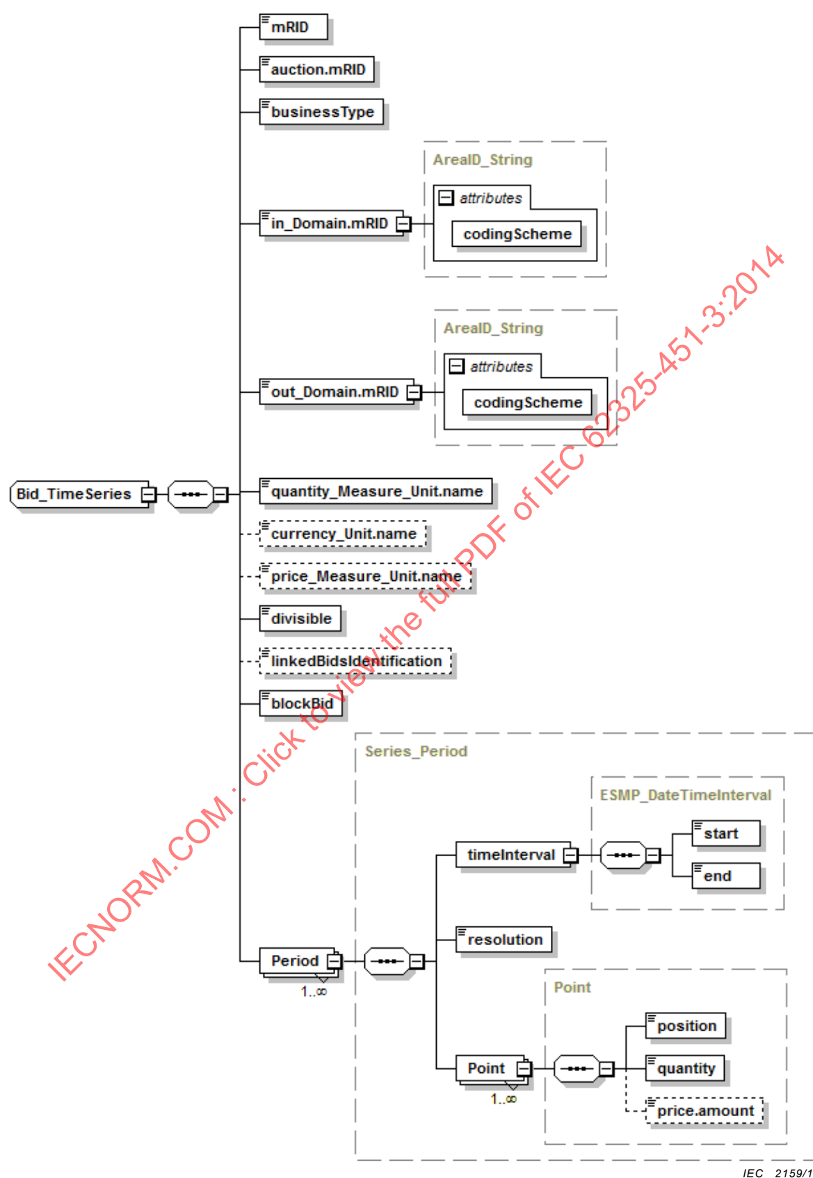
Figure 26 – Bid_MarketDocument XML schema structure – 2/2
