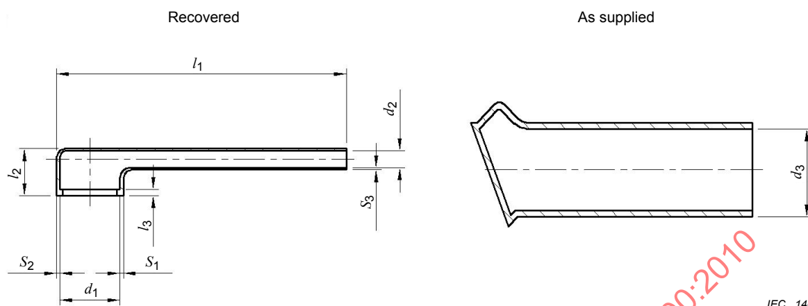
Figure 10 – Style I (lipped right-angle boot with longer tail)
