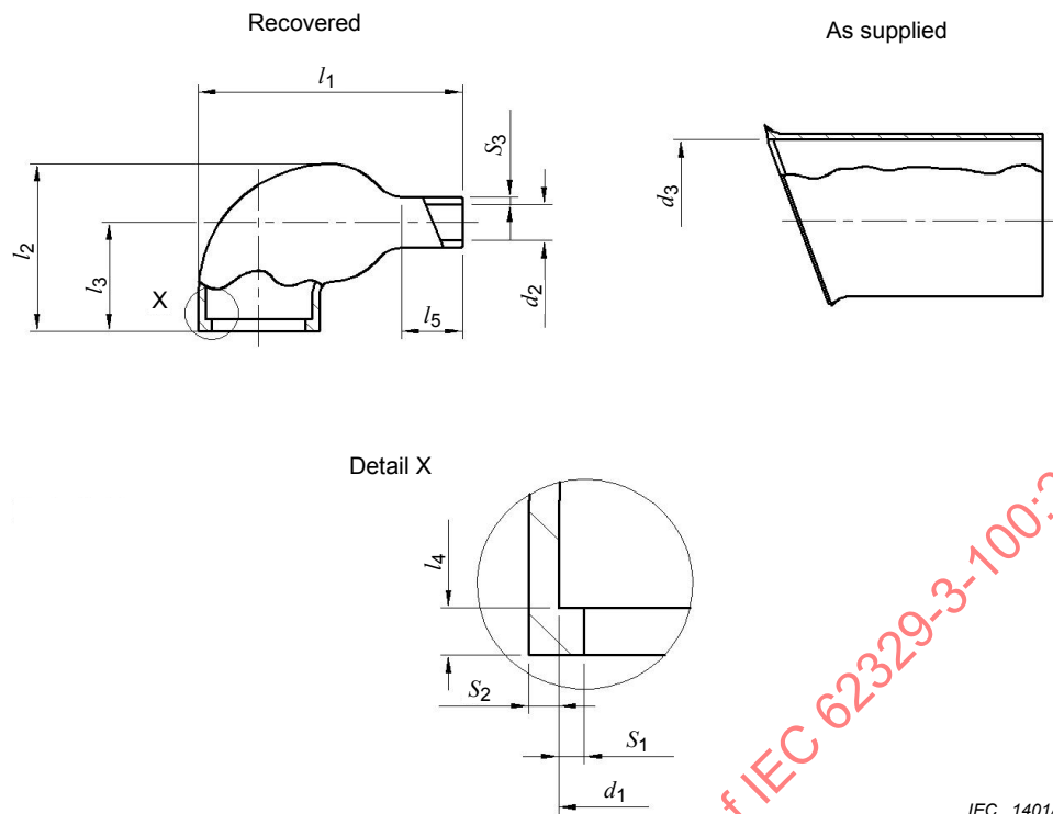
Figure 7 – Style F (lipped right-angle boot)
