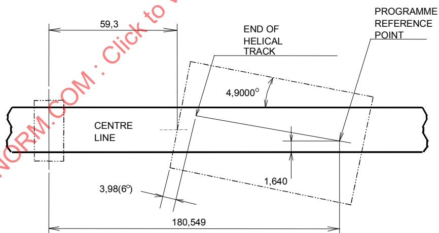
UNWRAPPED, VIEWED MAGNETIC COATING SIDE
