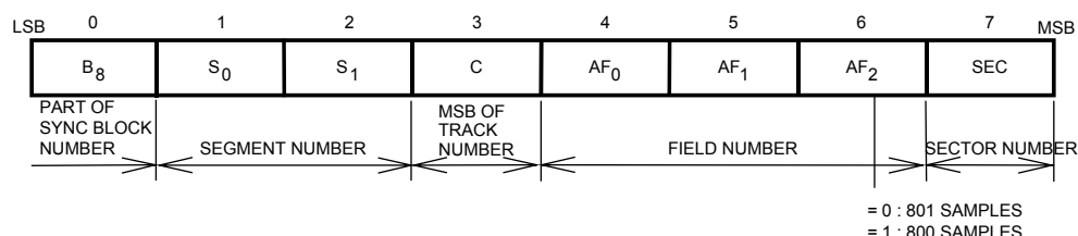
Figure 10 – Sync block identification format
