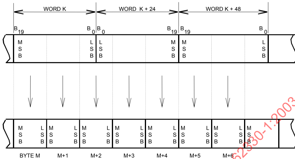
Figure 20 – Digital audio word to byte conversion
