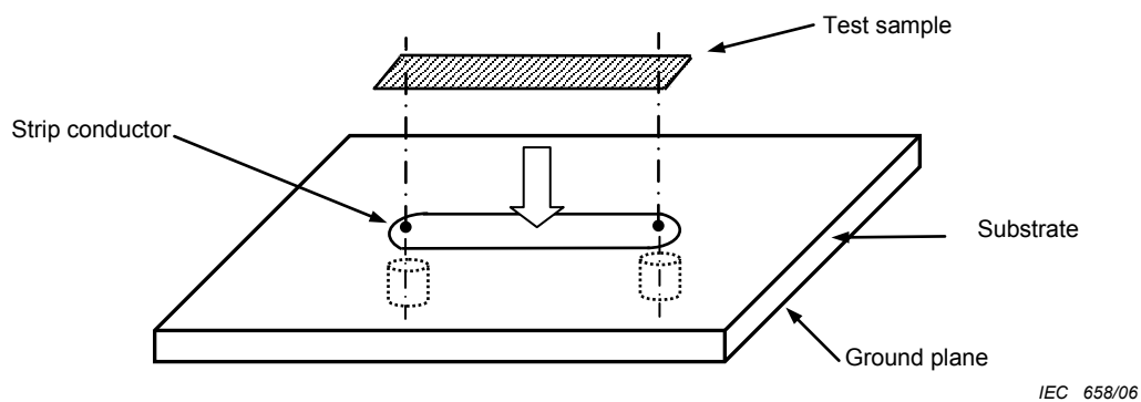
Figure 15 – Test sample attachment on test fixture
