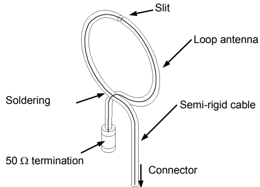
Figure 4b – Shielded loop antenna with slit and 50 Ω termination
