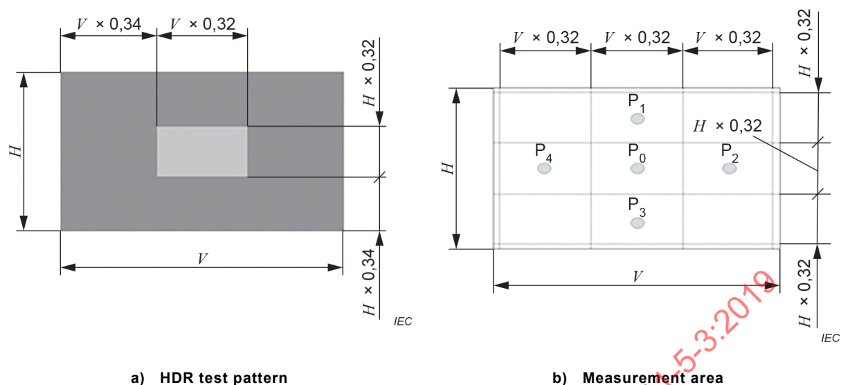
Figure 4 – Test pattern for HDR displays
