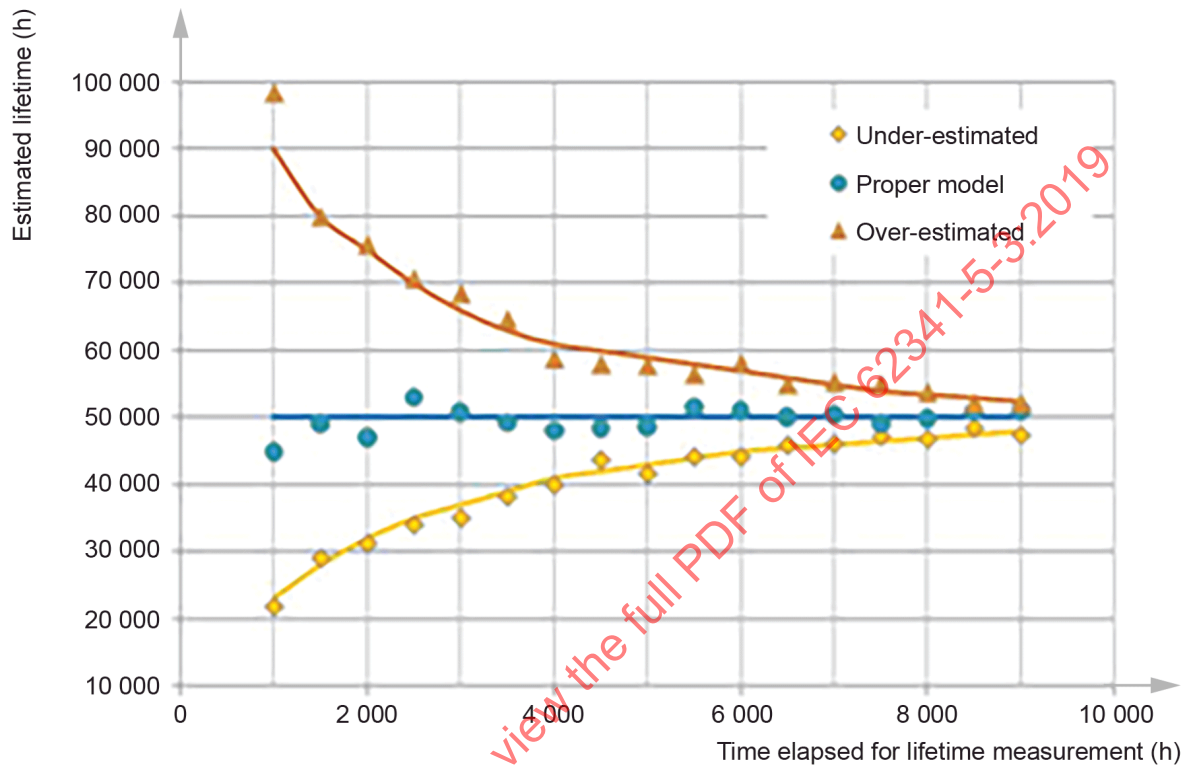
Figure 8 – Examples of estimated lifetime depending on the time elapsed
