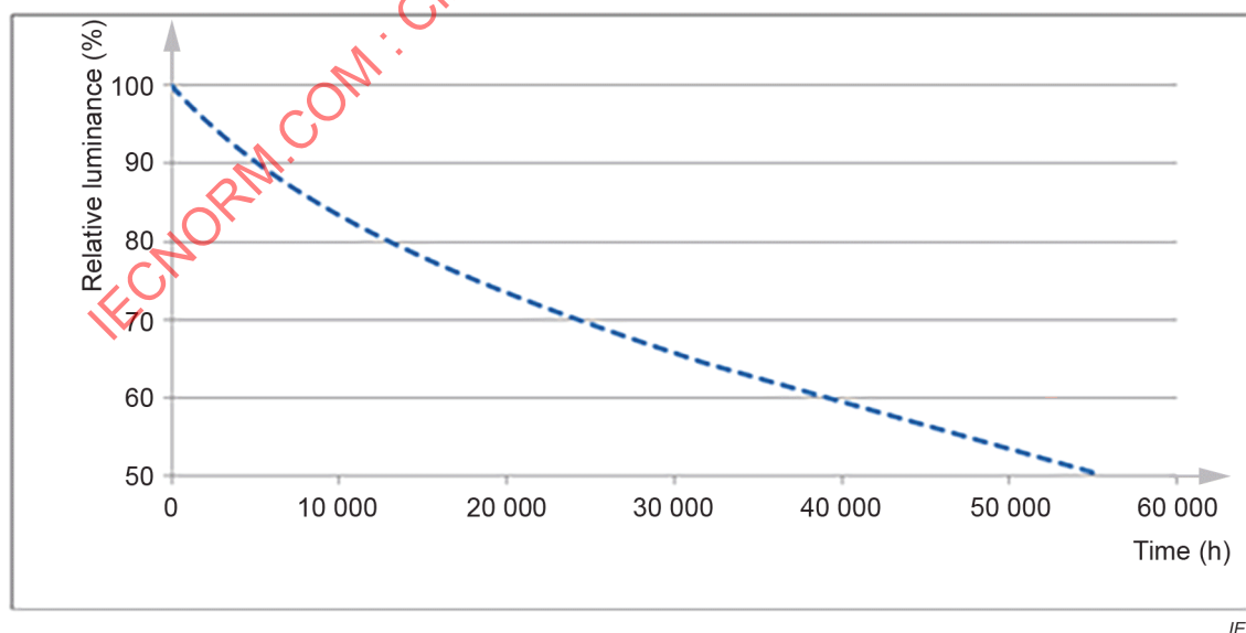
Figure 6 – Example of luminance behavior in operation for an OLED display module
