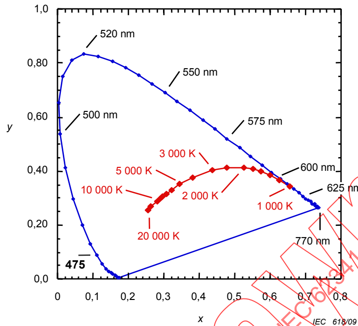
Figure 5 – Colour of blackbody source at various temperatures
