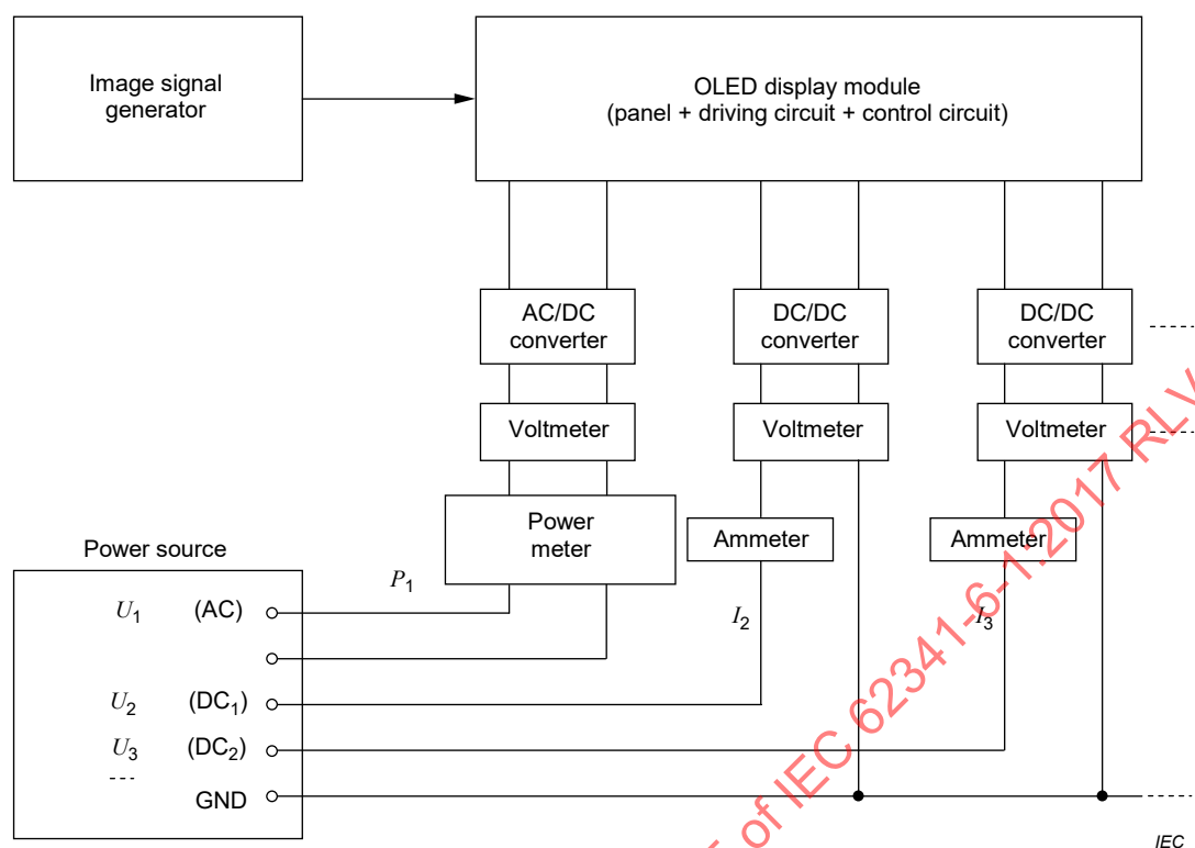
Figure 12 – Example of measurement setup of power consumption
