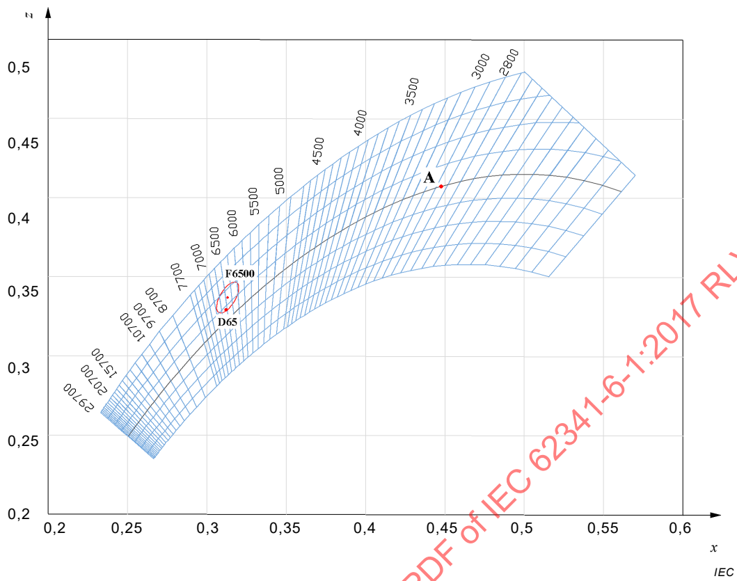
Figure D.2 – Blackbody locus (Planckian locus) and isotherm lines in CIE 1931 XYZ chromaticity diagram
