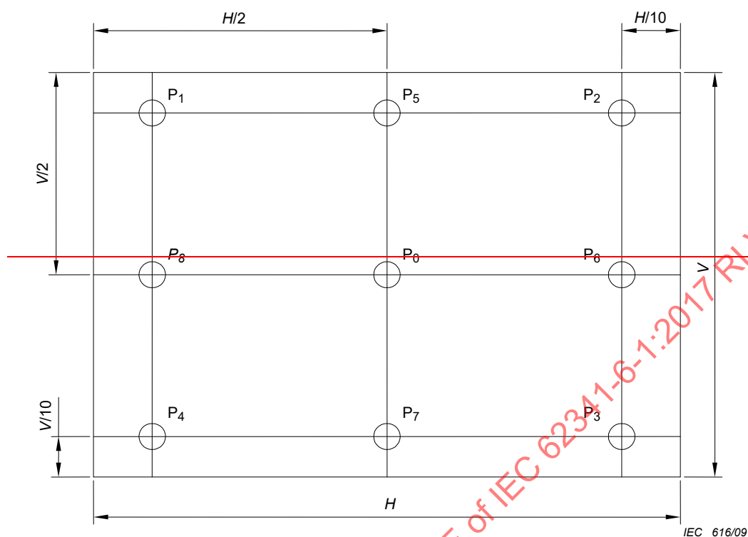
Figure 3 – Measurement points
