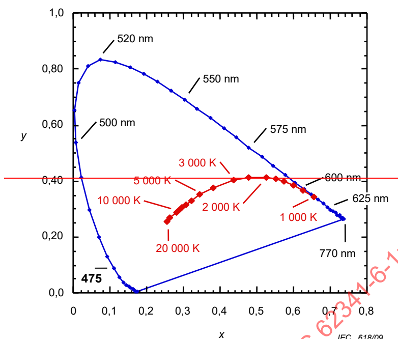
Figure 5 — Colour of blackbody source at various temperatures
