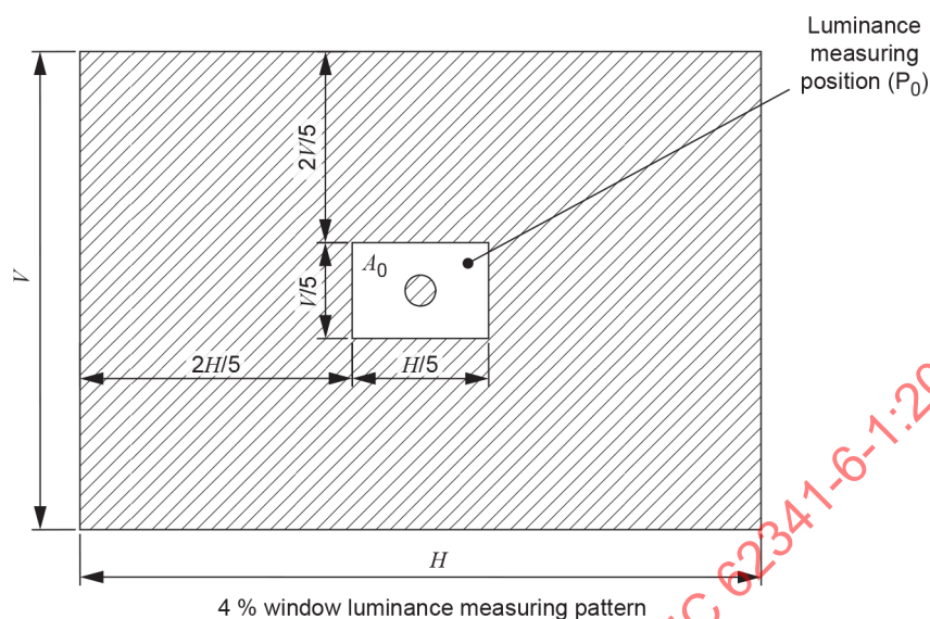
Figure F.1 – Example of simple 4 % white window pattern at the centre of the screen
