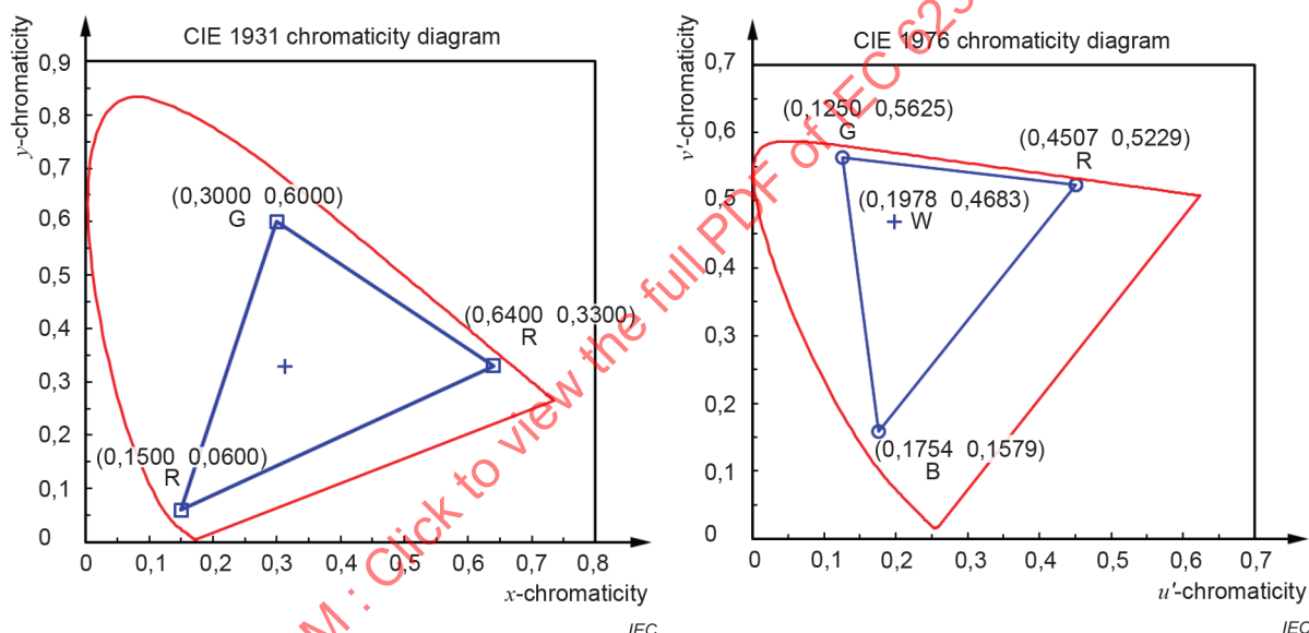
Figure 10 – Example of representation of the same primary colours in the CIE 1931 (left) and CIE 1976 (right) chromaticity diagrams
