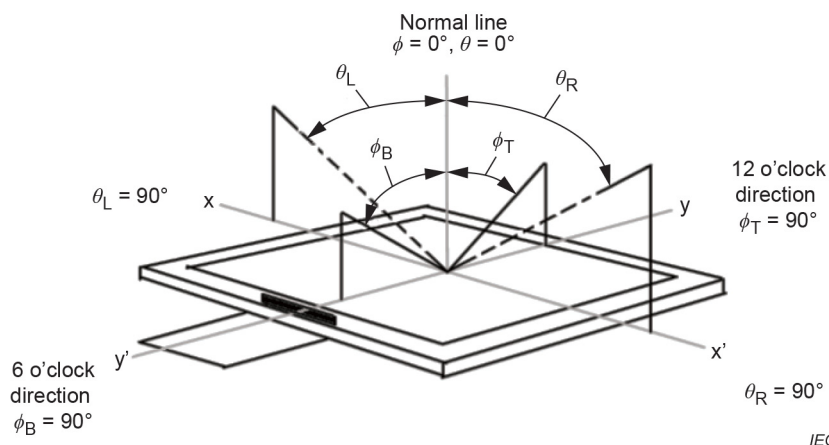
Figure 4 – Viewing angle set up
