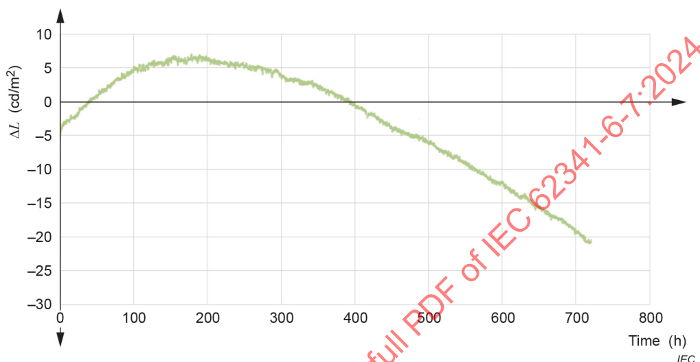
Figure 6 – Example of the decrease of a luminance difference curve
