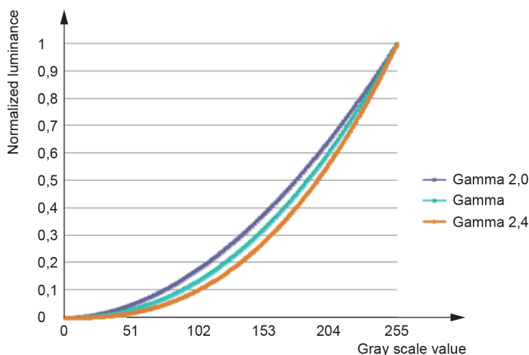
Figure 3 – Example tone curve of the display
