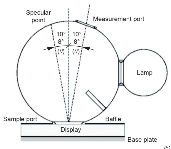
Figure 2 – Measurement geometries for reflectance
