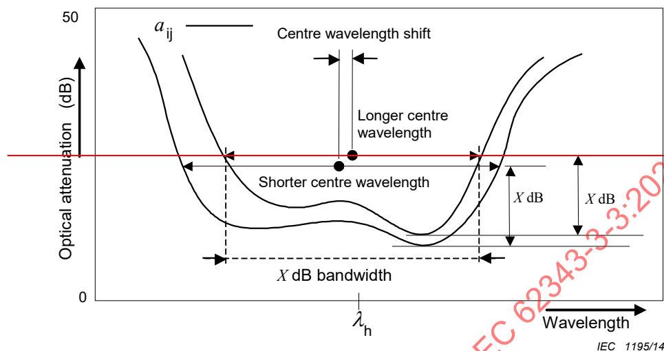
Figure 1 — Illustration of X -dB bandwidth
