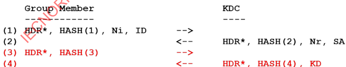
Figure 38 – GROUPKEY-PULL Key Download Exchange
