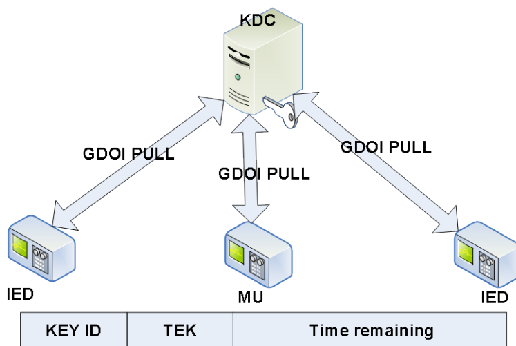
Figure 4 – GDOI Pull Phase 2
