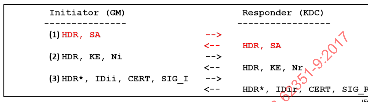
Figure 21 – IKEv1 main mode exchange and security association messages
