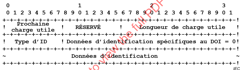
Figure 30 – Charge utile Identification (RFC 6407)
