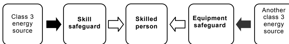
Figure 19 – Model for protection of a skilled person against class 3 energy sources during equipment servicing conditions
