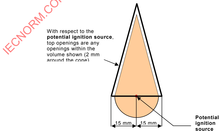
Figure 45 – Top openings
