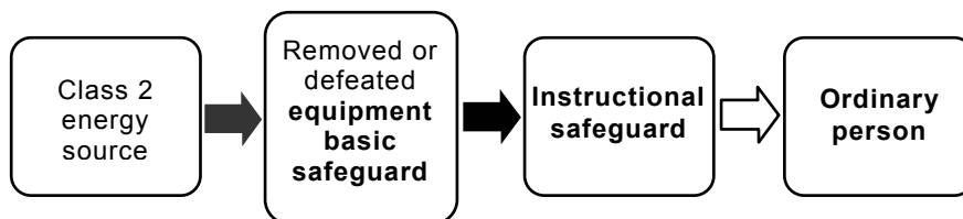
Figure 11 – Model for protection of an ordinary person against a class 2 energy source during ordinary person servicing conditions
