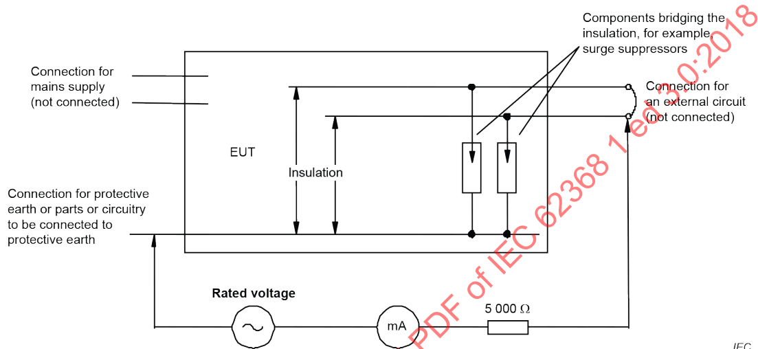
Figure 31 – Test for separation between an external circuit and earth
