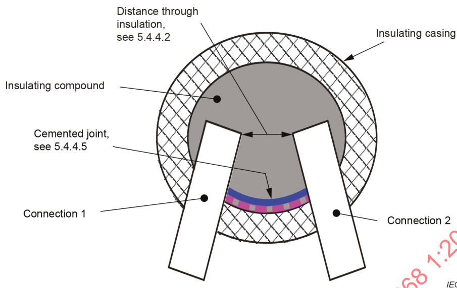
Figure O.15 – Device filled with insulating compound
