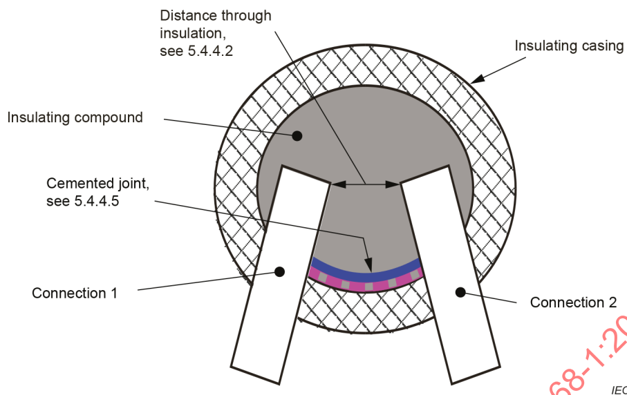
Figure O.15 – Device filled with insulating compound
