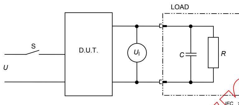
Figure A.1a – Test circuit for current during the starting process
