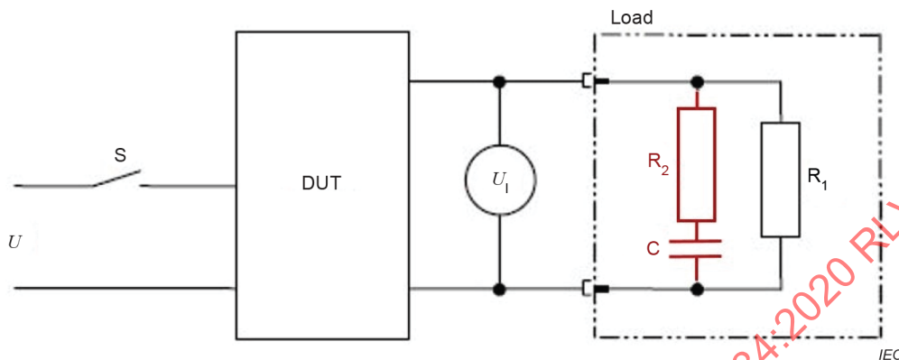
a) Test circuit for current during the starting process
