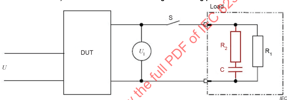
b) Test circuit for current when connecting the load during the steady state operation
