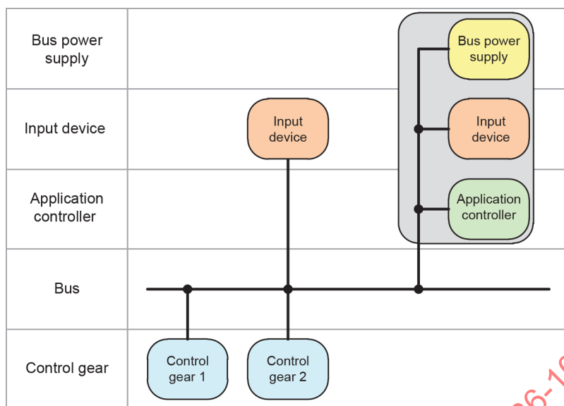
Figure A.5 – Multi-master architecture example with integrated input device and bus power supply
