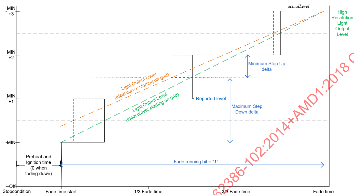
Figure B.1 – Level behaviour in cases of off-grid starting points
