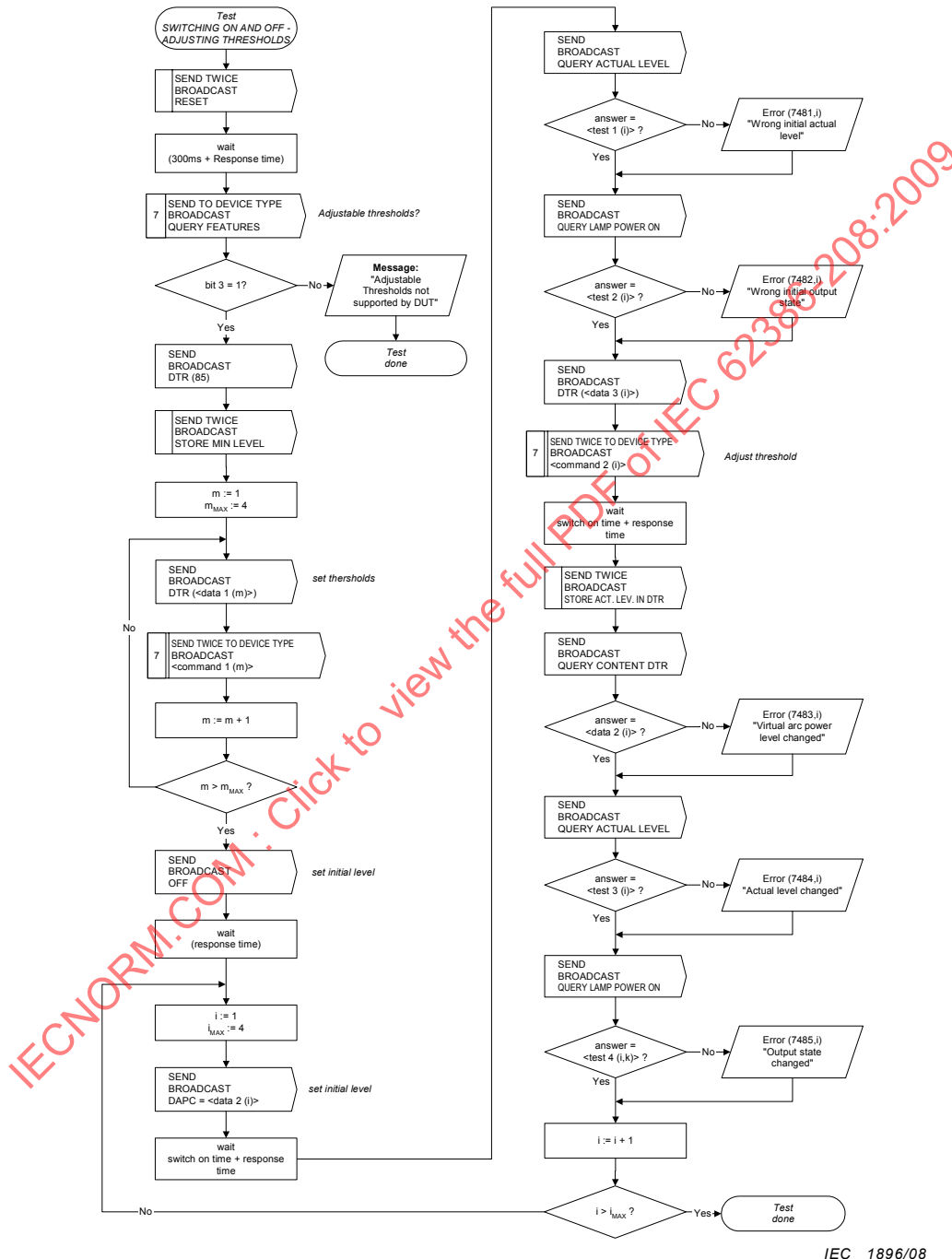
Figure 31 – Test sequence SWITCHING ON AND OFF – ADJUSTING THRESHOLDS
