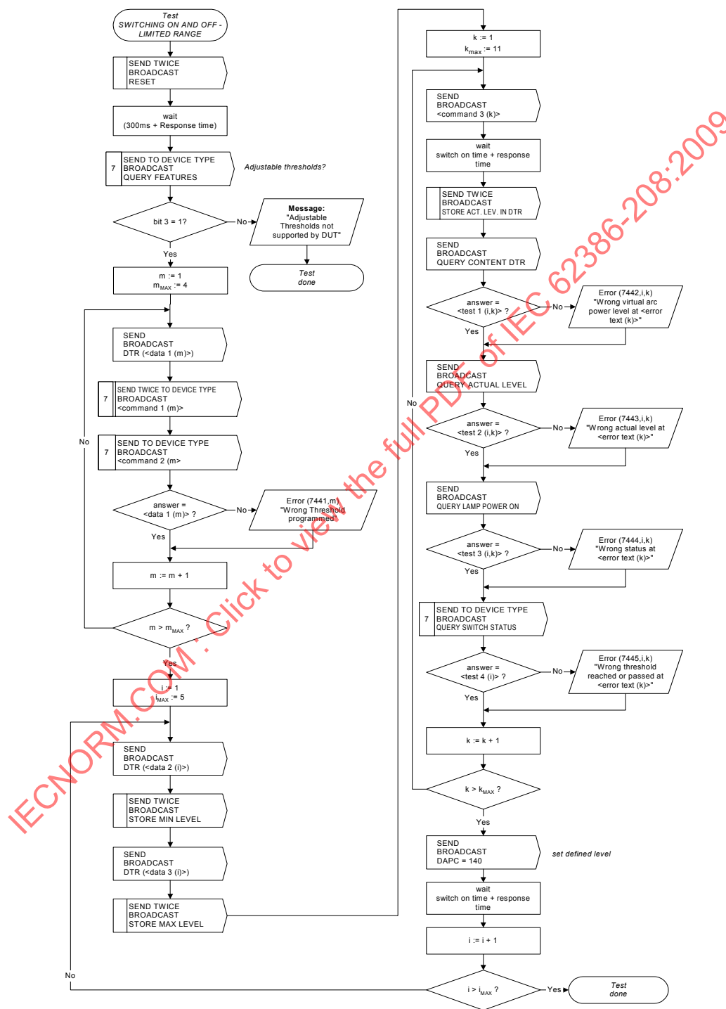
Figure 27 – Test sequence SWITCHING ON AND OFF – LIMITED RANGE
