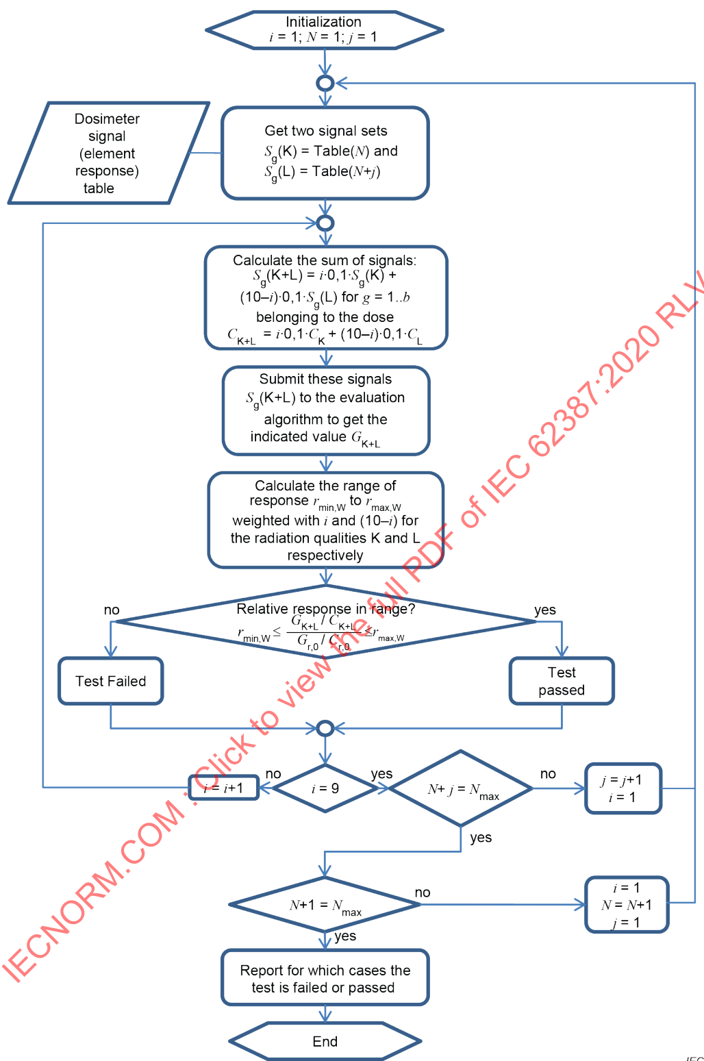
Figure F.1 – Flow chart of a computer program to perform tests according to 12.2
