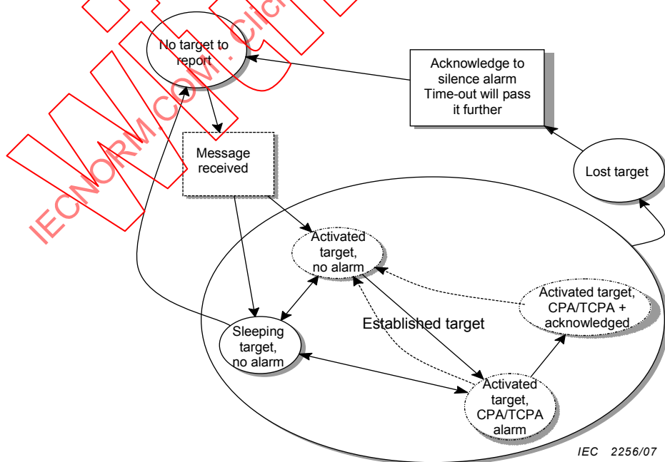
Figure G.2 – AIS target states
