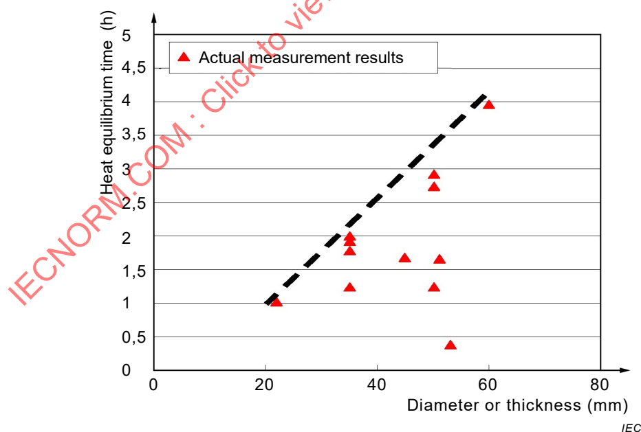
Figure C.1 – Thermal equilibrium times of capacitors (from 85 °C to 25 °C)
