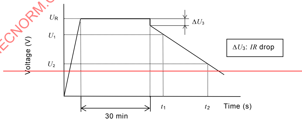
Figure 2 – Voltage characteristic between capacitor terminals
