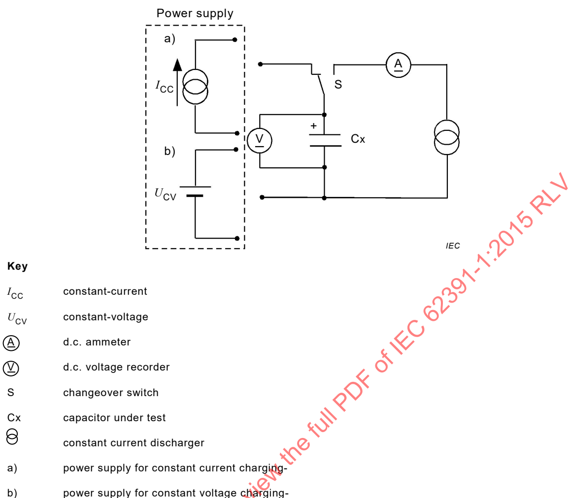
Figure 1 – Basic circuit for measuring
