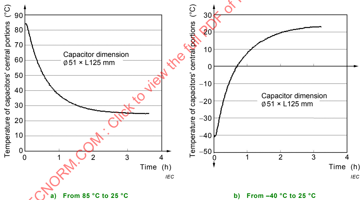
Figure C.2 – Thermal equilibrium times of capacitors (from -40\text{ }^{\circ}\text{C} to 25\text{ }^{\circ}\text{C} )
