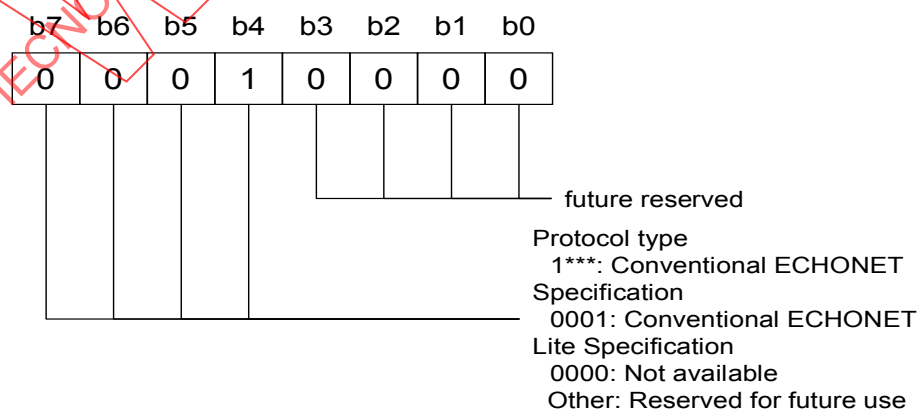
Figure 32 – Detailed specifications of ELHD1
