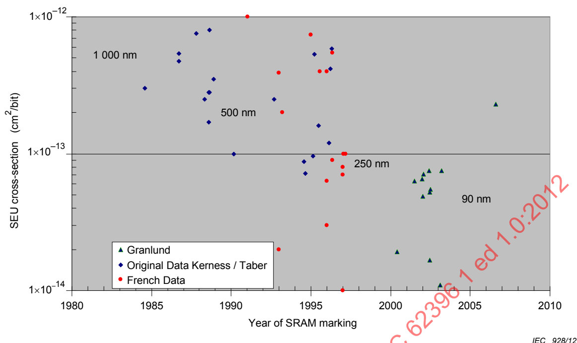
Figure 10 – SEU cross-section in SRAMs as function of manufacture date
