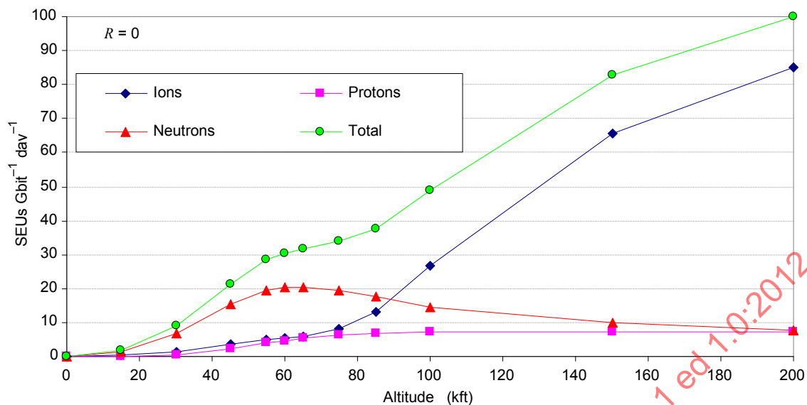
Figure E.6 – Calculated contributions from neutrons, protons and heavy ions to the SEU rates of the Hitachi-A 4 Mbit SRAM as a function of altitude at a cut-off rigidity ( R ) of 0 GV
