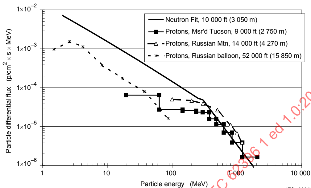
Figure 5 – Energy spectrum of protons within the atmosphere
