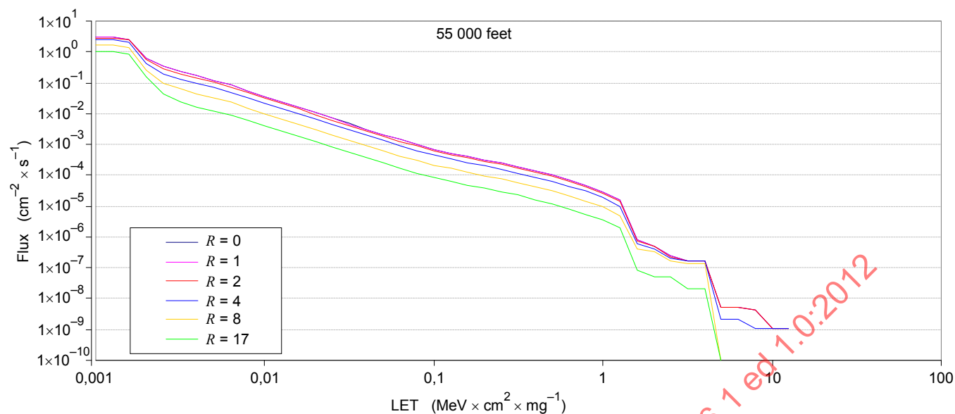
Figure E.3 – Integral linear energy transfer spectra in silicon at 55 000 feet (16 760 m) for cut-off rigidities ( R ) from 0 GV to 17 GV
