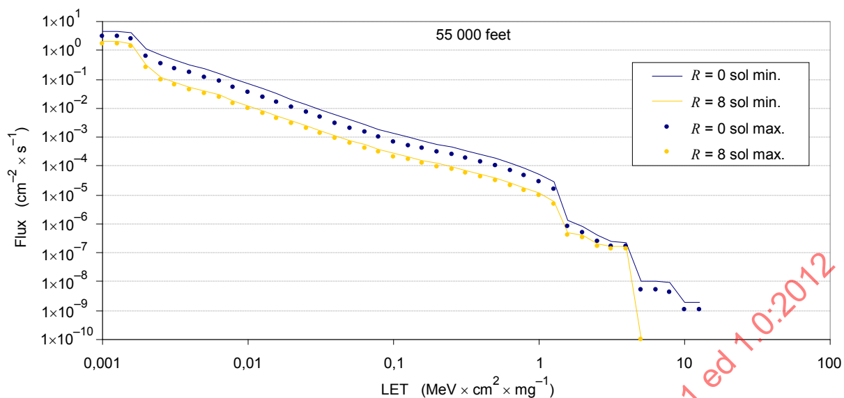
Figure E.5 – The influence of solar modulation on integral linear energy transfer spectra in silicon at 55 000 feet (16 760 m) for cut-off rigidities ( R ) of 0 GV and 8 GV
