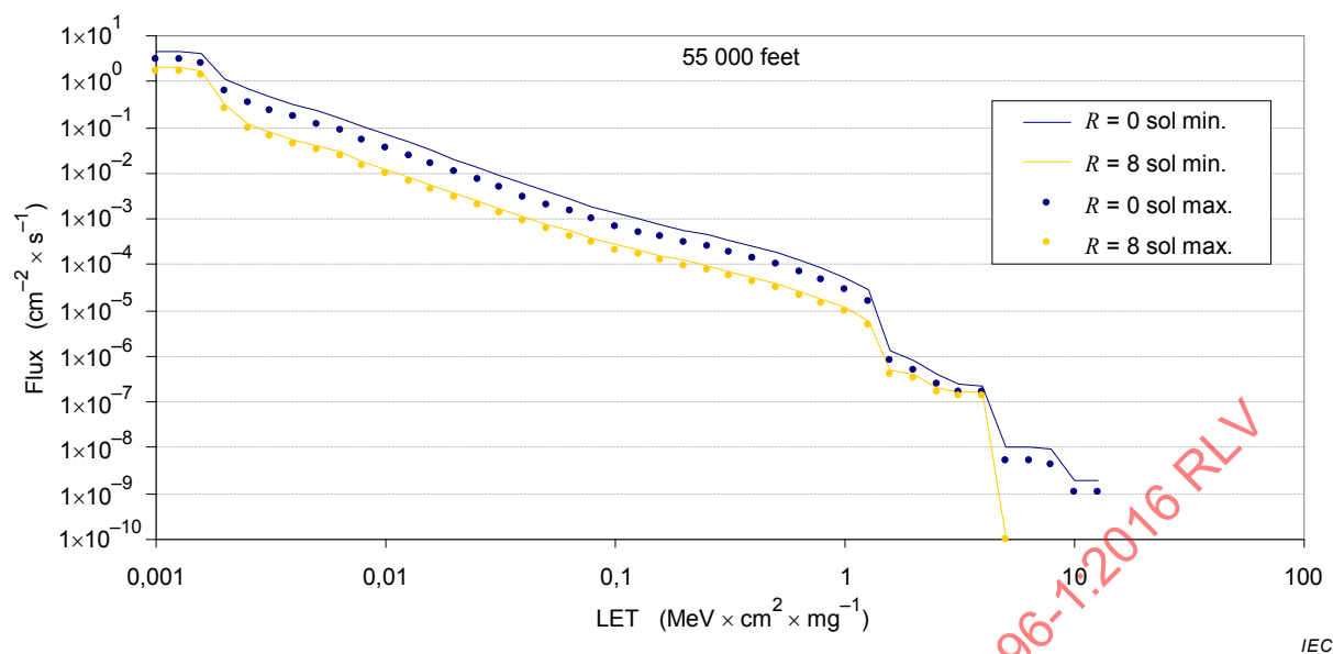
Figure E.5 – The Influence of solar modulation on integral linear energy transfer spectra in silicon at 55 000 ft (16 760 m) for cut-off rigidities ( R ) of 0 GV and 8 GV
