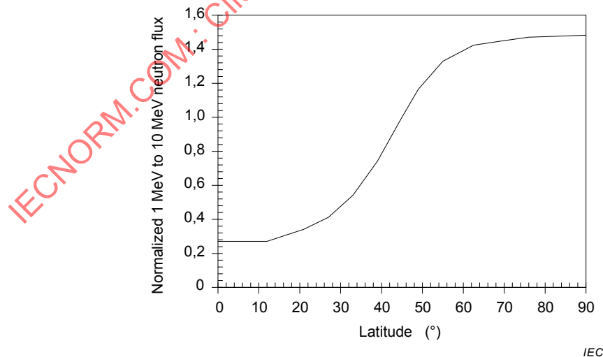
Figure 4 – Model of atmospheric neutron flux variation with latitude
