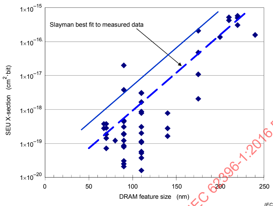
Figure G.2 – Variation of the high energy neutron SEU cross-section per bit as a function of electronic device feature size for DRAMs
