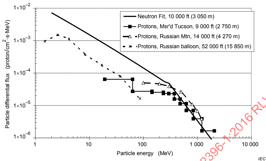
Figure 5 – Energy spectrum of protons within the atmosphere
