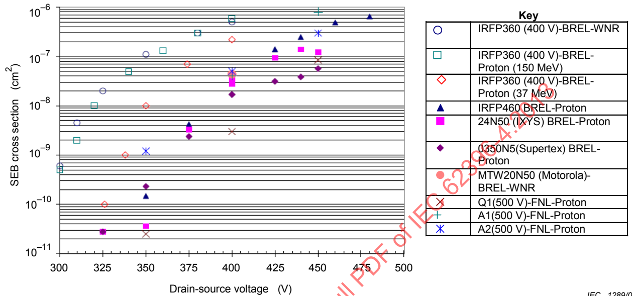
Figure 1 – SEB cross sections measured in 400 V and 500 V MOSFETs for WNR neutron and proton beams
