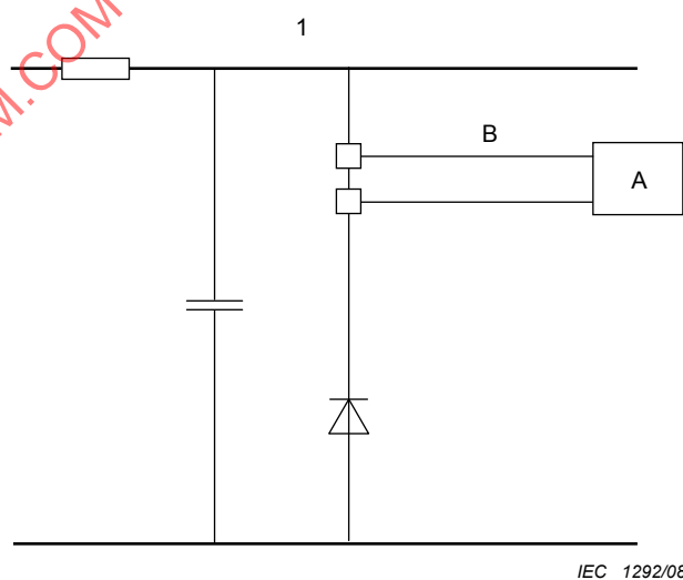
b) Application of EPICS to the measurement of radiation event induced current
