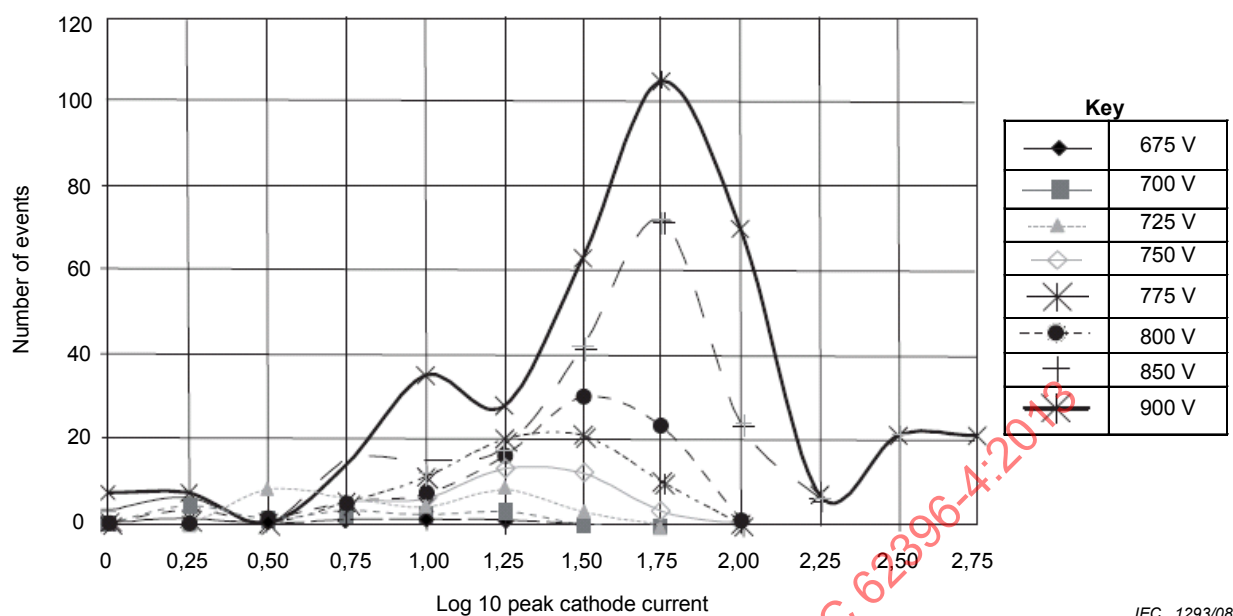
Figure 4 – EPICS plot of 1 200 V diode numbers of events at currents taken at different applied voltages for a neutron fluence of approximately 3,5 \times 10^9 neutrons per \text{cm}^2 measured at energies greater than 10 MeV
