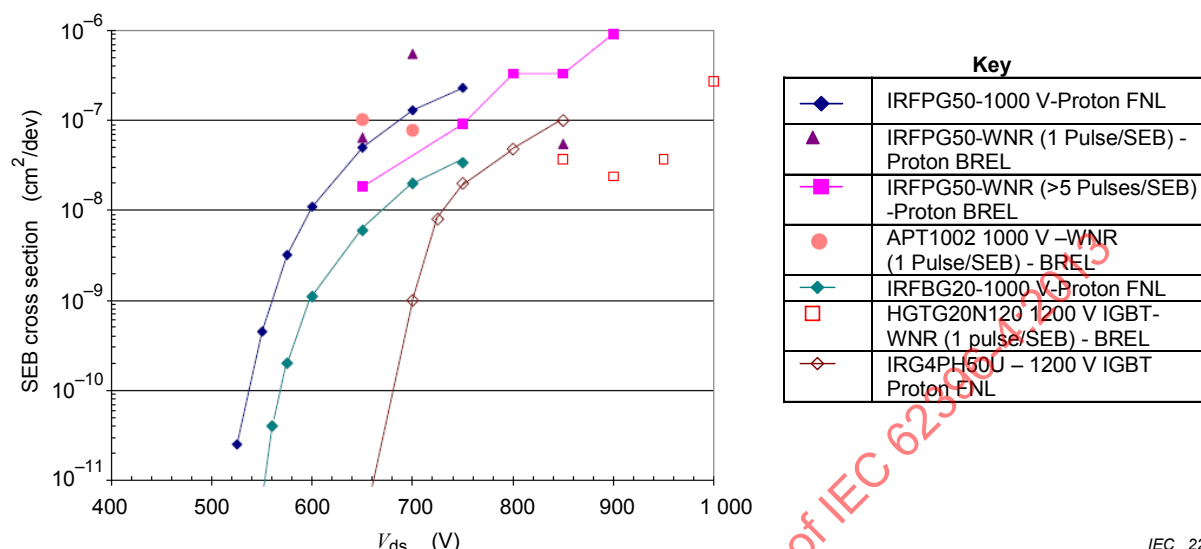
Figure 2 – SEB cross sections measured in 1 000 V MOSFETs and 1 200 V IGBTs with WNR neutron and 200 MeV proton beams
