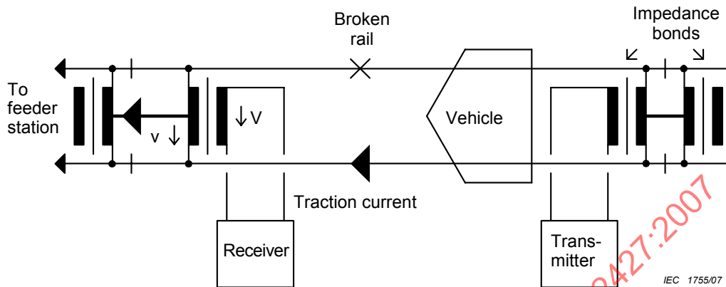
Figure A.5 – Double rail track circuit with broken rail
