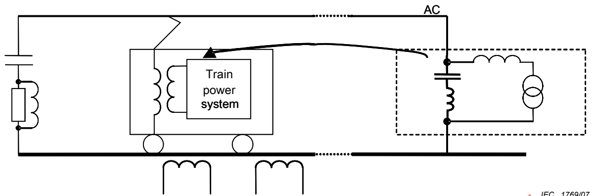
Figure E.4 – Circulation of interference current generated by the substation
