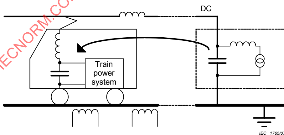
Figure D.3 – Circulation of interference current generated by the substation
