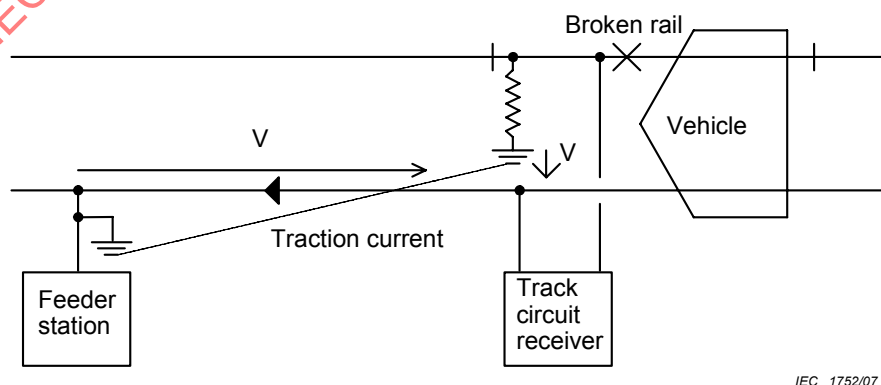
Figure A.2 – Interference mechanism with self-revealing broken rail
