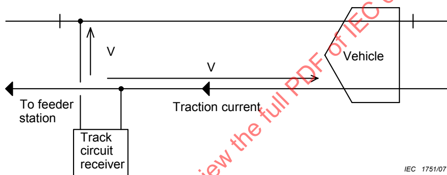
Figure A.1 – Interference mechanism with intact rails
