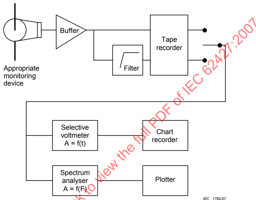
Figure B.1 – Example of a system for the measurement of interference currents
