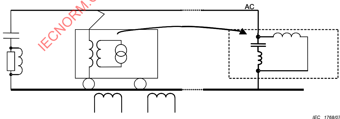
Figure E.2 – Rolling stock and AC supply with power converter
