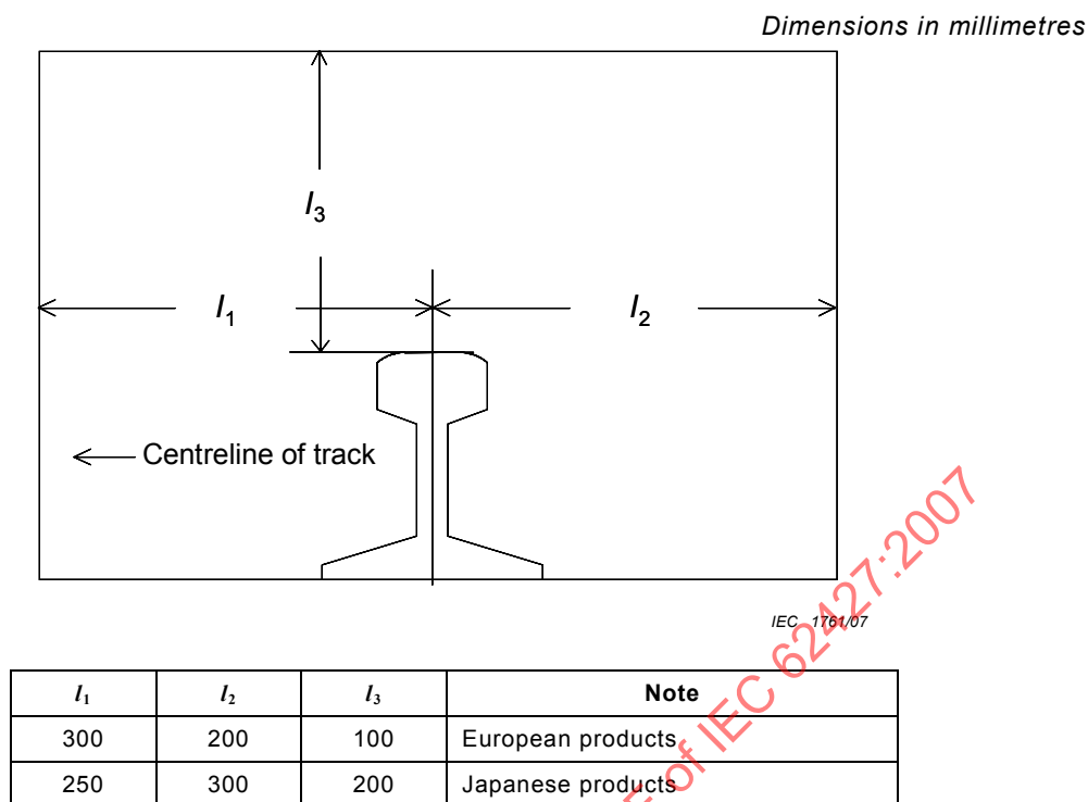
Figure A.11 – Sensitive zone of wheel detectors
