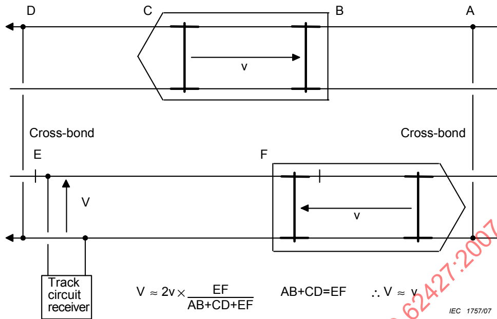
Figure A.7 – Interference mechanism due to voltage between axles – Case 2
