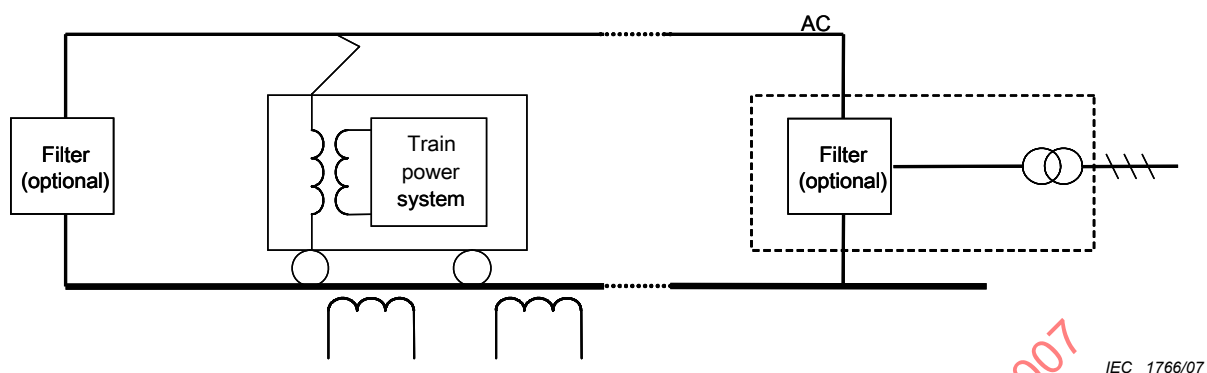
Figure E.1 – Rolling stock and AC supply without power converter
