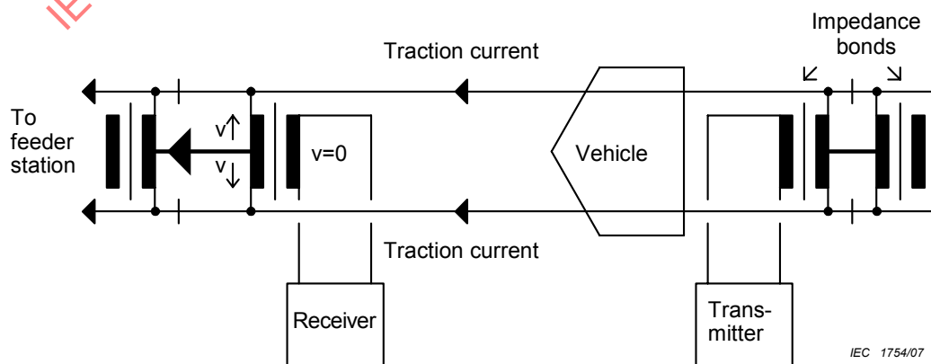
Figure A.4 – Double rail track circuit
