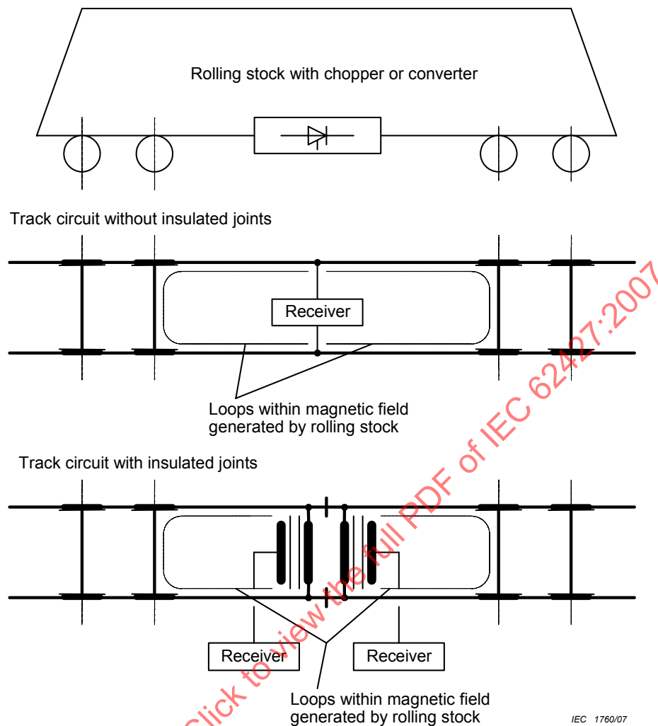
Figure A.10 – Example of radiated interference
