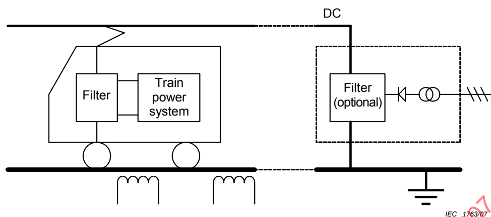
Figure D.1 – Rolling stock with DC supply
