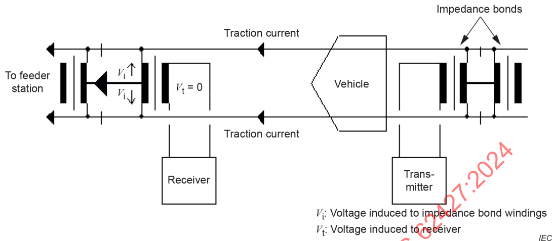
Figure A.4 – Double rail track circuit
