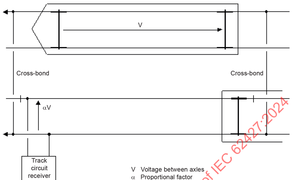
Figure A.6 – Interference mechanism due to voltage between axles – Case 1
