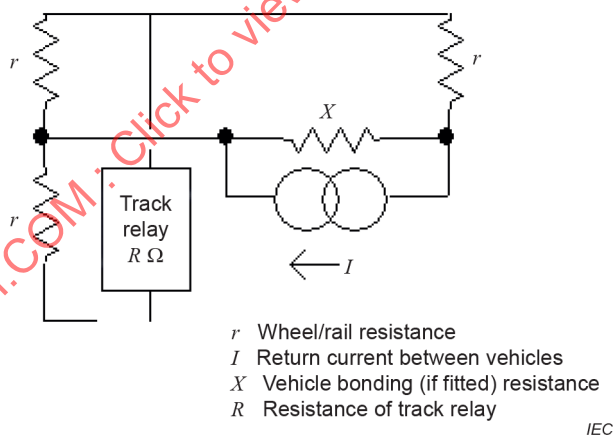
Figure A.9 – Equivalent circuit for Figure A.8
