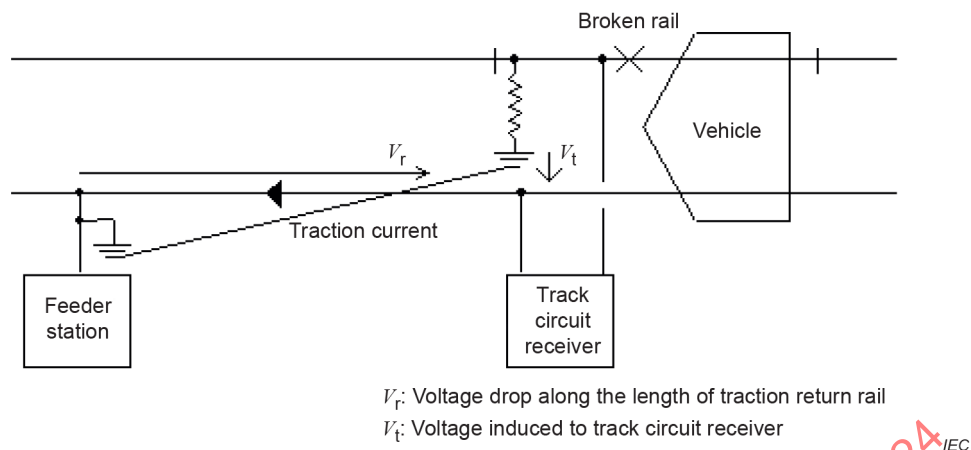
Figure A.2 – Interference mechanism with self-revealing broken rail
