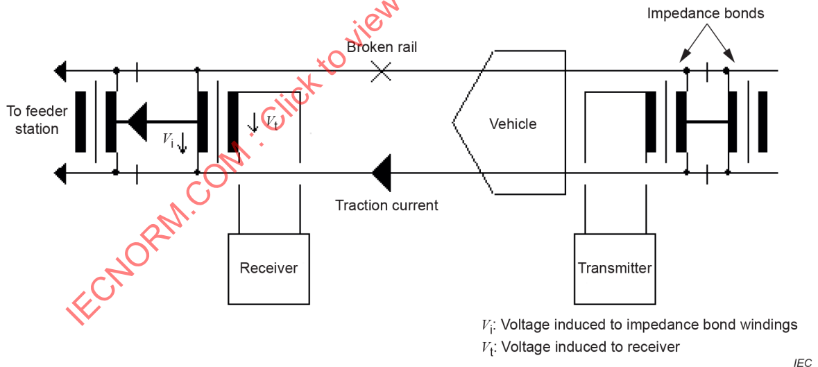
Figure A.5 – Double rail track circuit with broken rail
