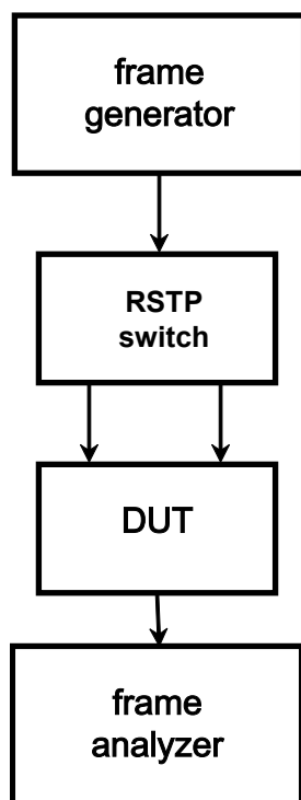
Figure 20 –Test rig for T_L measurement
