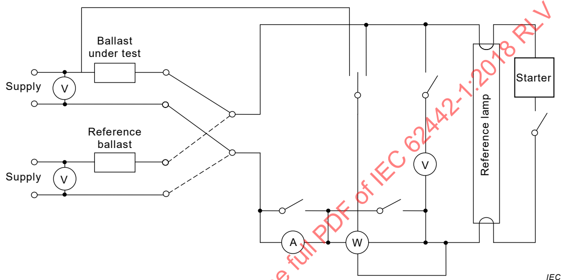
Figure A.1 – Measurement of magnetic wire wound electromagnetic controlgear-lamp circuits
