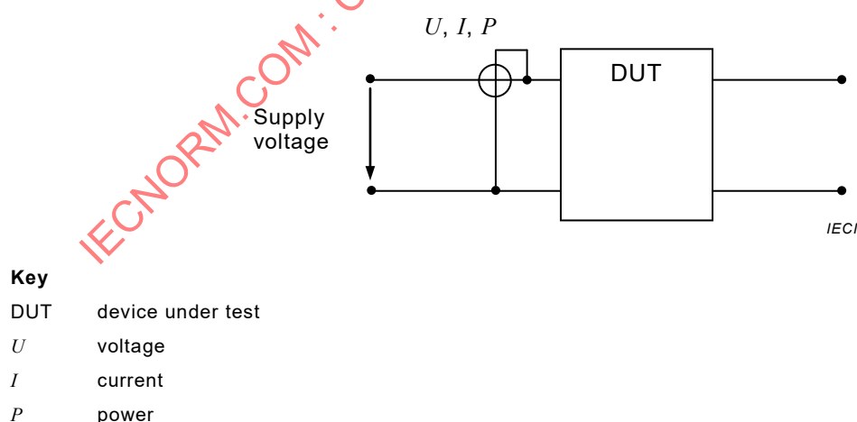
Figure 2 – Input power in no-load mode measurement setup for electromagnetic controlgear (transformer) and for converter (electronic controlgear)
