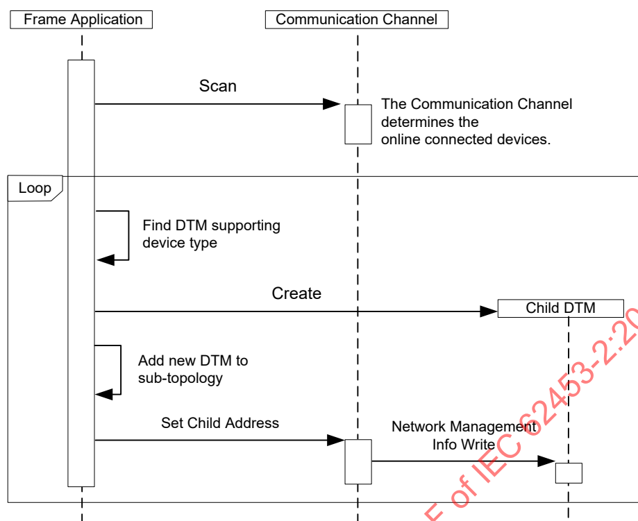
Figure 46 – Scanning and DTM assignment
