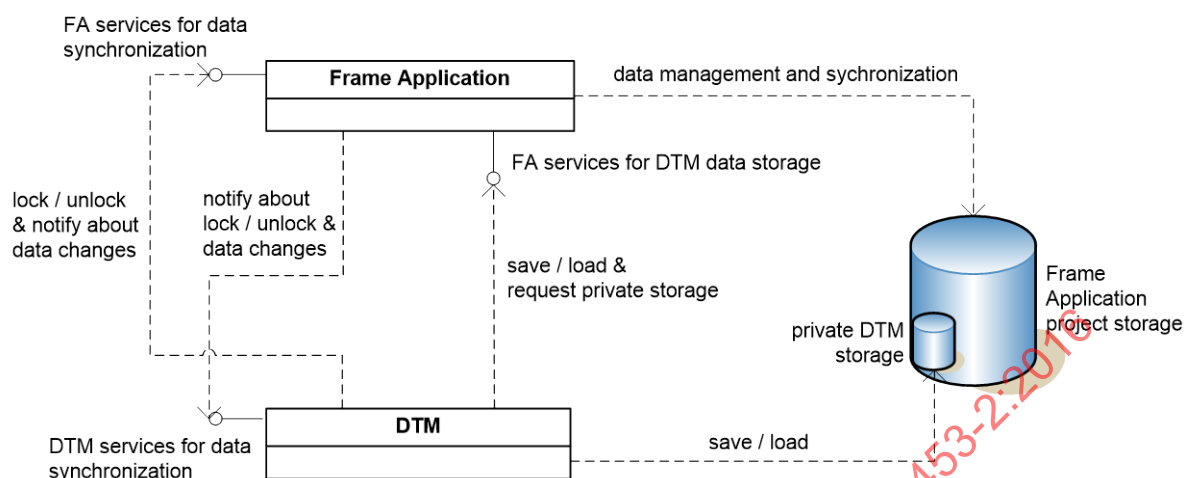
Figure 22 – FDT storage and synchronization mechanisms
