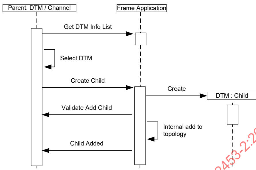
Figure 39 – FDT topology generation triggered by a DTM
