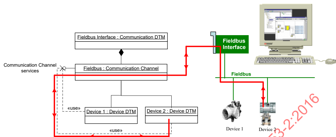
Figure 18 – Point-to-point communication
