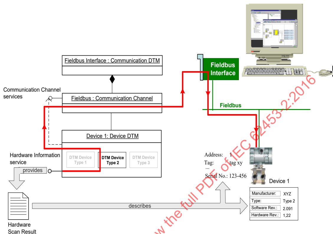
Figure 21 – Connected Hardware Identification
