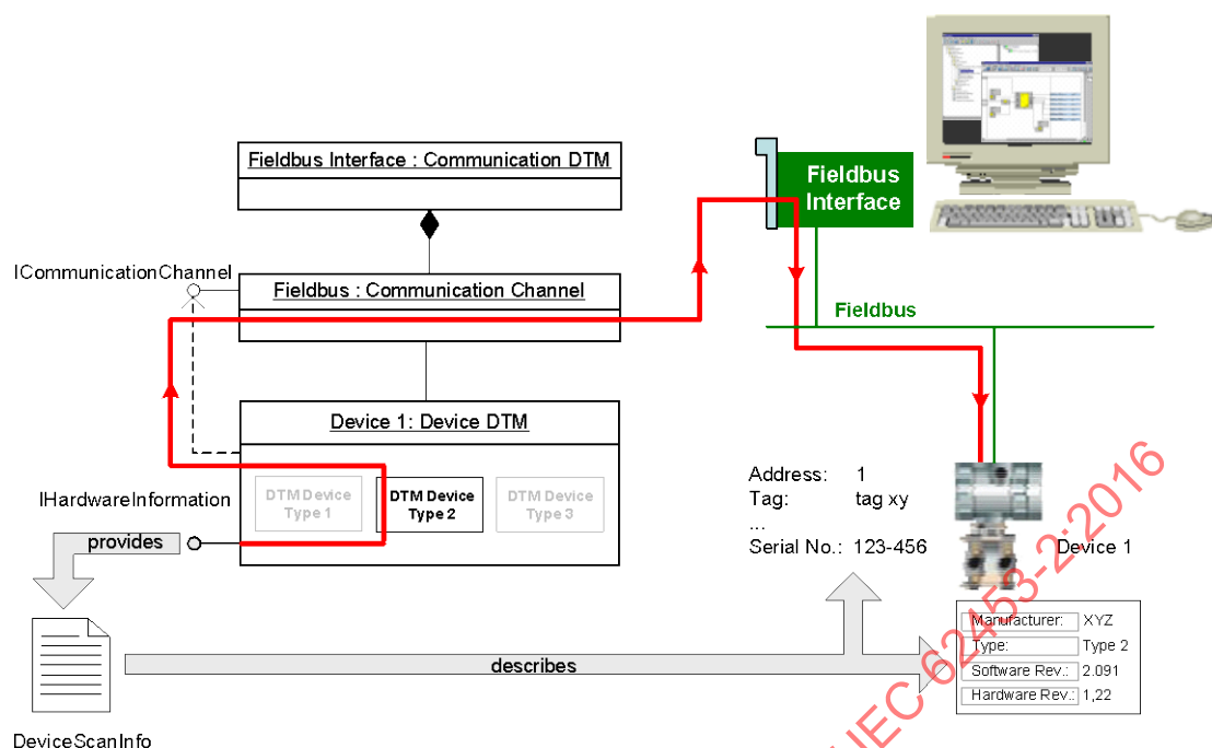
Figure 15 – Identification of connected devices
