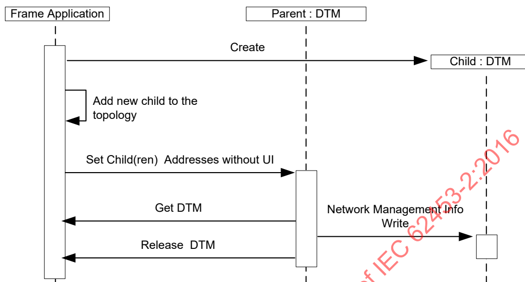
Figure 41 – Set or modify device address – without user interface
