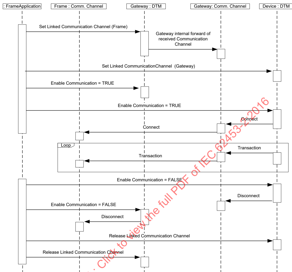
Figure 44 – Nested communication
