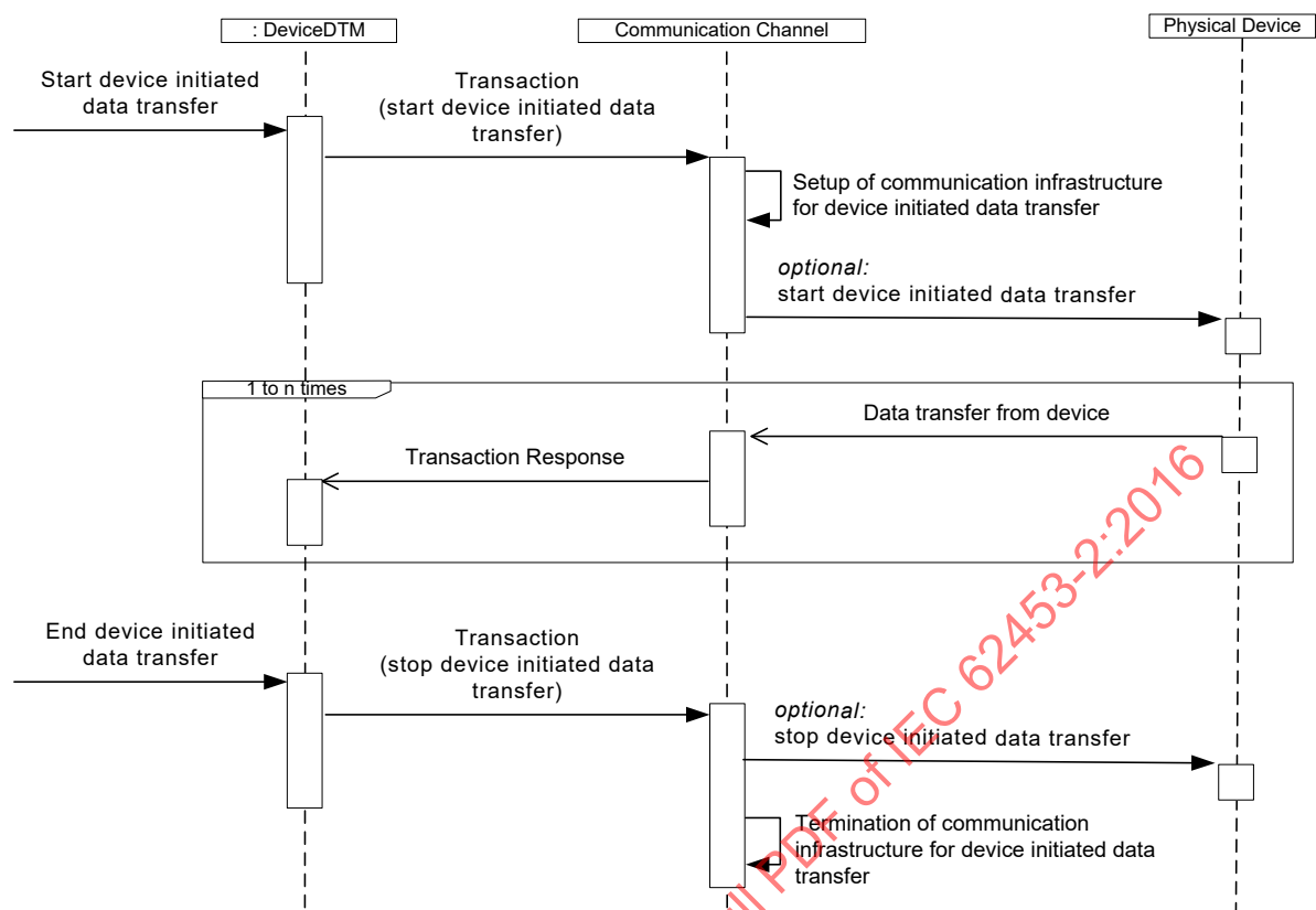
Figure 45 – Device initiated data transfer
