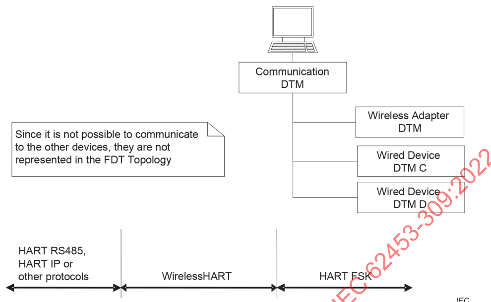
Figure 10 – FDT Topology when directly connected to a WirelessHART adapter device
