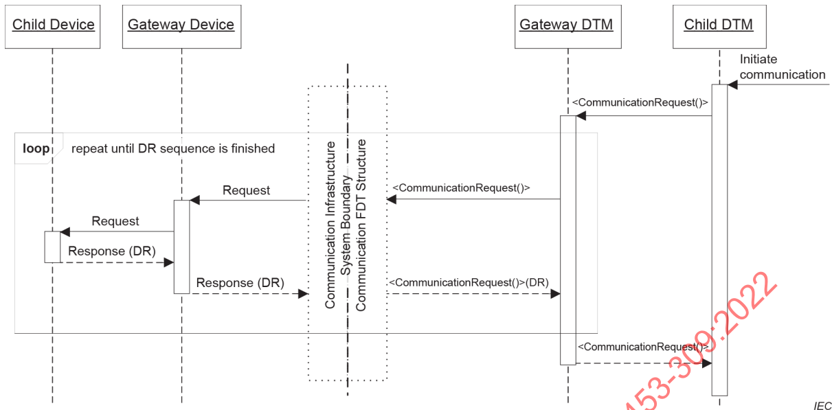
Figure 4 – Handling of delayed responses (scenario 2)
