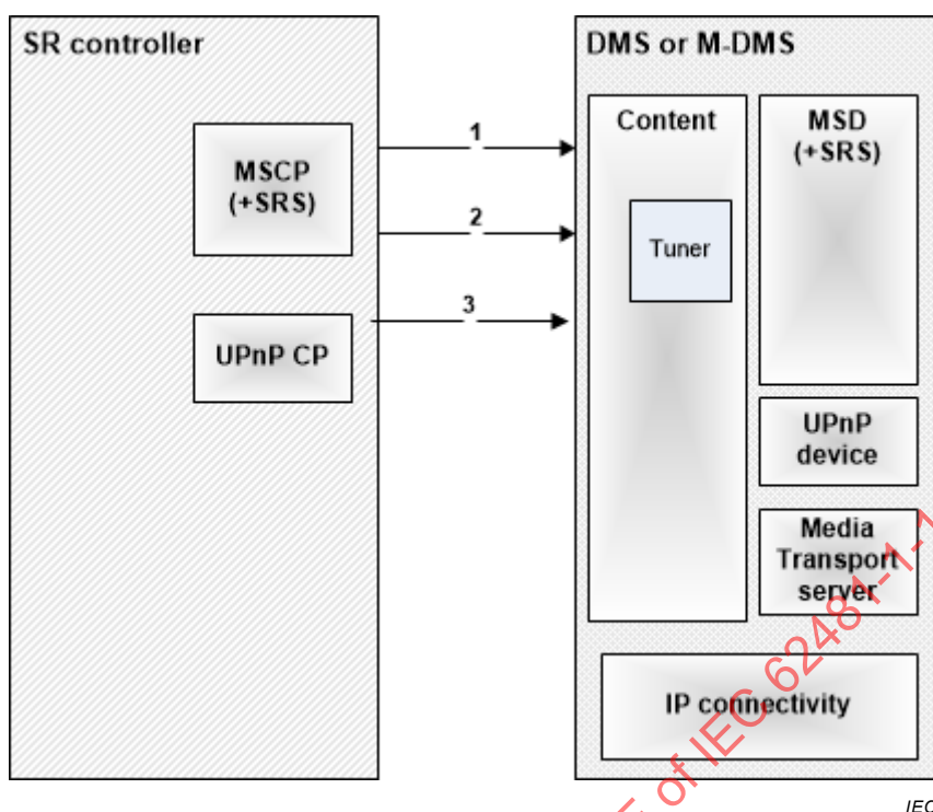
Figure 10 – Scheduled Recording system usage interaction model
