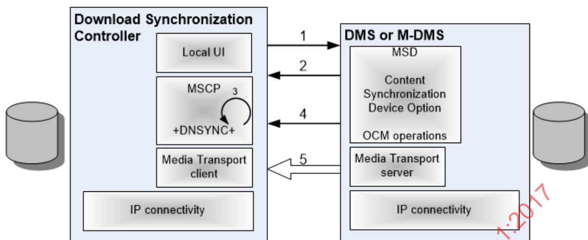
Figure 8 – Download Synchronization system usage interaction model
