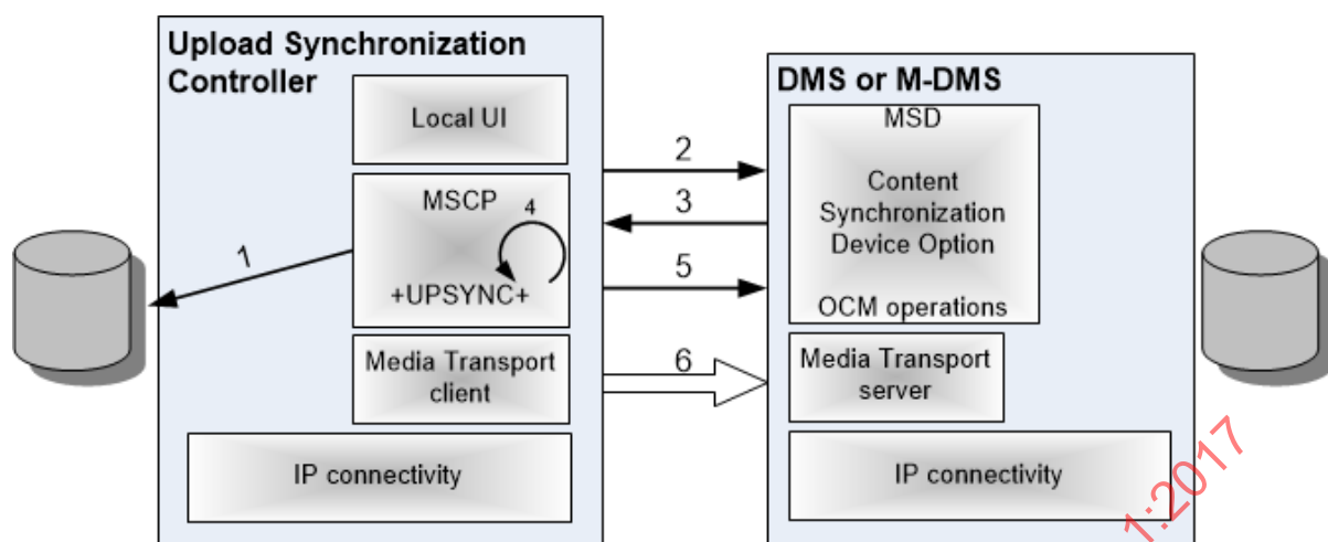
Figure 9 – Upload Synchronization system usage interaction model
