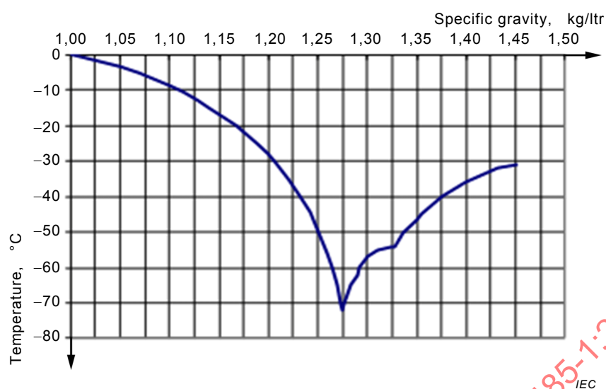
Figure 4 – Freezing point curve of sulphuric acid
