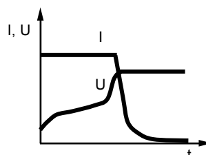
Figure A.4 – IU-or CC-CV charge profile Figure A.5 – Time dependant profile of current I and voltage U
