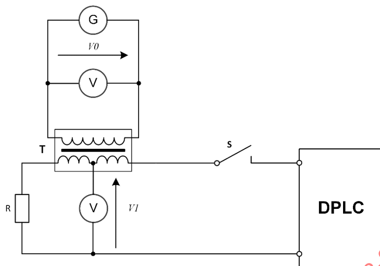
Figure 10 – Test circuit for return loss measurement
