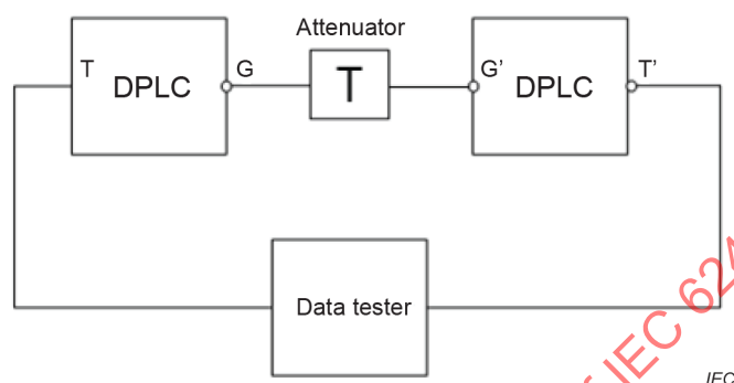
Figure 17 – Test circuit for serial data transmission delay measurement with a data tester
