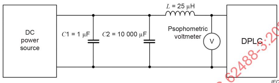
Figure 20 – LF disturbances measurement setup
