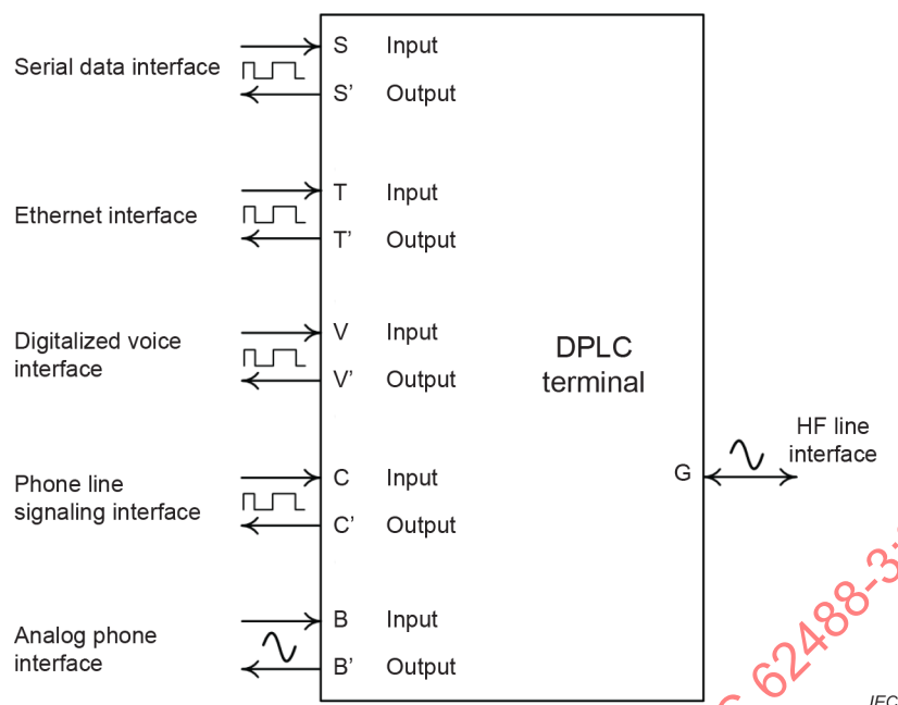
Figure 8 – Reference points for measuring DPLC parameters
