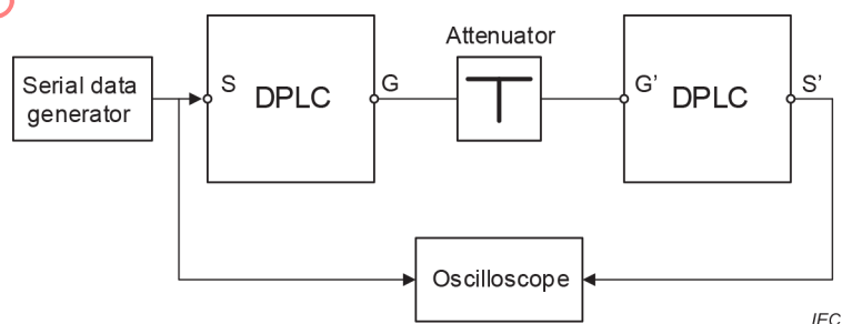
Figure 18 – Test circuit for serial data transmission delay measurement
