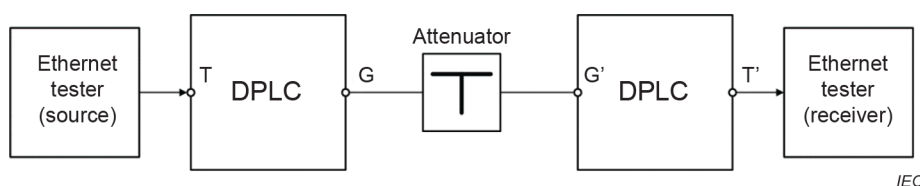
Figure 19 – Test circuit for maximal throughput and latency measurement
