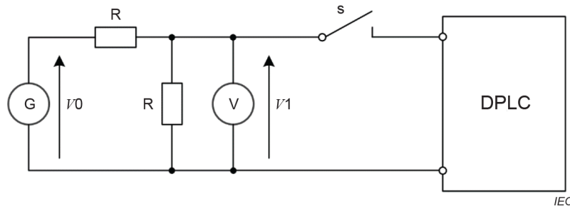
Figure 13 – Test circuit for tapping loss measurement
