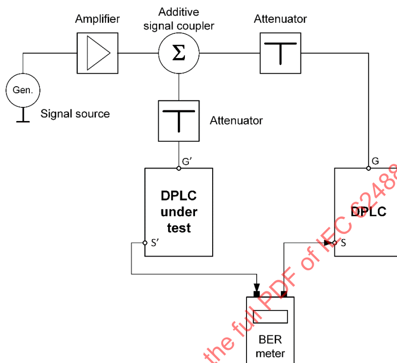
Figure 15 – Test circuit for selectivity measurement
