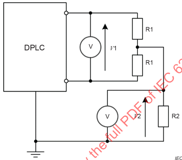
Figure 12 – Test circuit for OSB measurement (Rx port)
