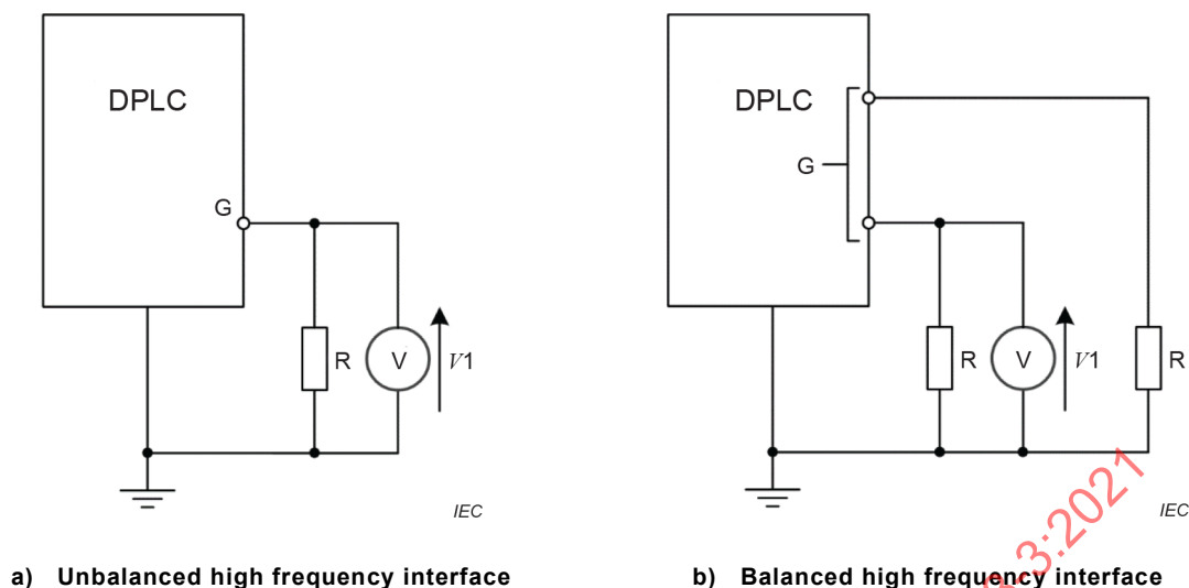
Figure 14 – Test circuit for spurious and in-band emissions measurement
