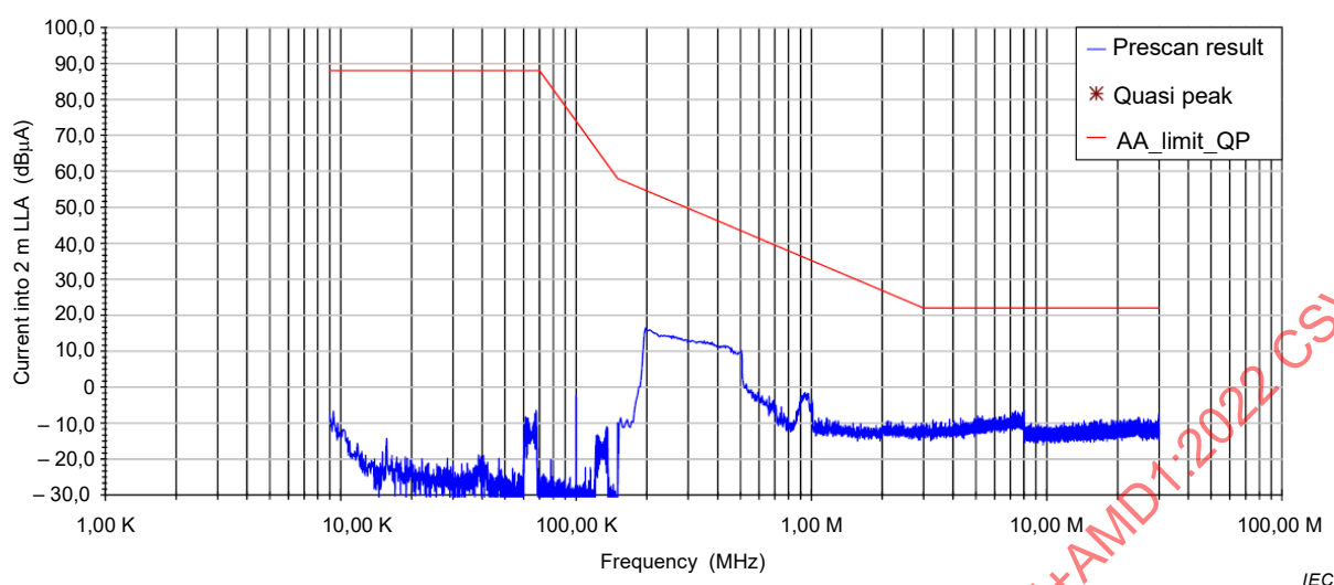
Figure D.5 – Example of magnetic-field test result using the LLA
