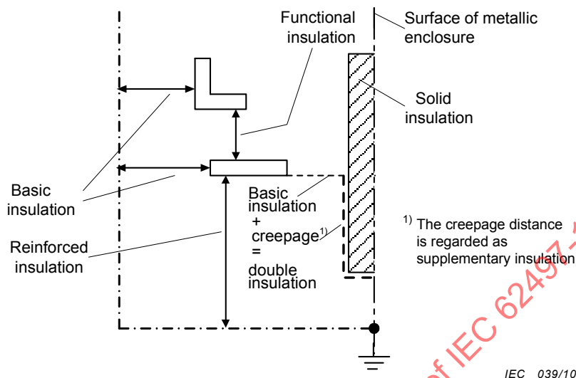
Figure F.2 – Example for types of insulation
