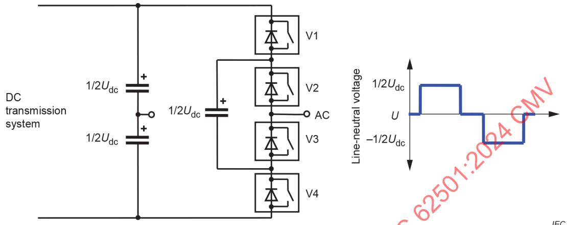
Figure A.7 – Basic circuit topology of one phase unit of a 3-level flying capacitor converter
