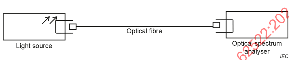
Figure B.3 – Measurement set-up for signal to total source spontaneous emission ratio
