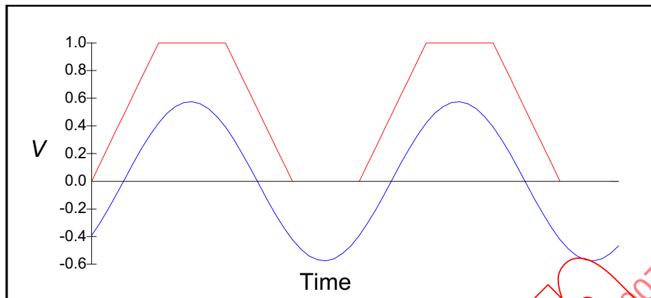
Figure B.16—BandPass (response of Filter to TrapezoidVoltage)
