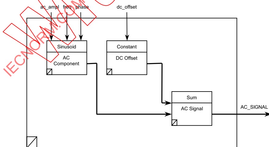
Figure E.1—TSF AC_SIGNAL
