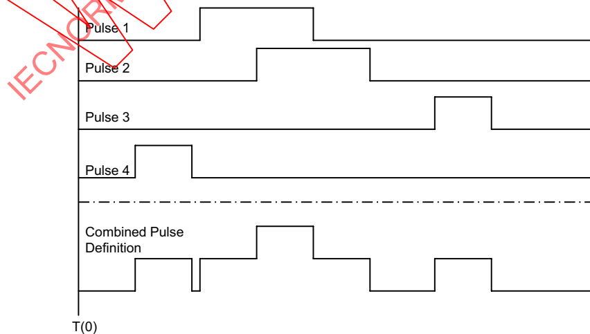
Figure B.3—Pulses using PulseDefns
