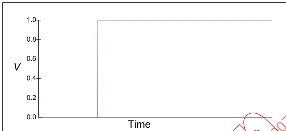
Figure B.5—Step (amplitude = 1 V, startTime = 0.5 s)
