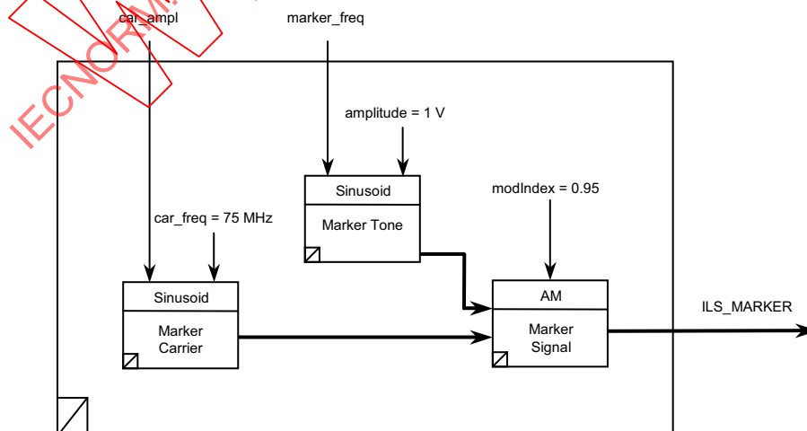
Figure E.21—TSF ILS_MARKER
