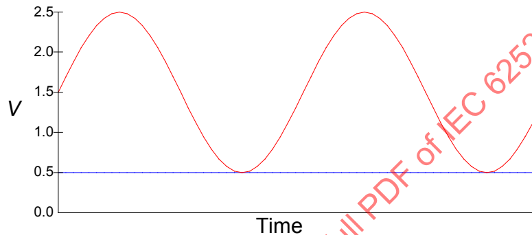
Figure B.55—MinInstantaneous
