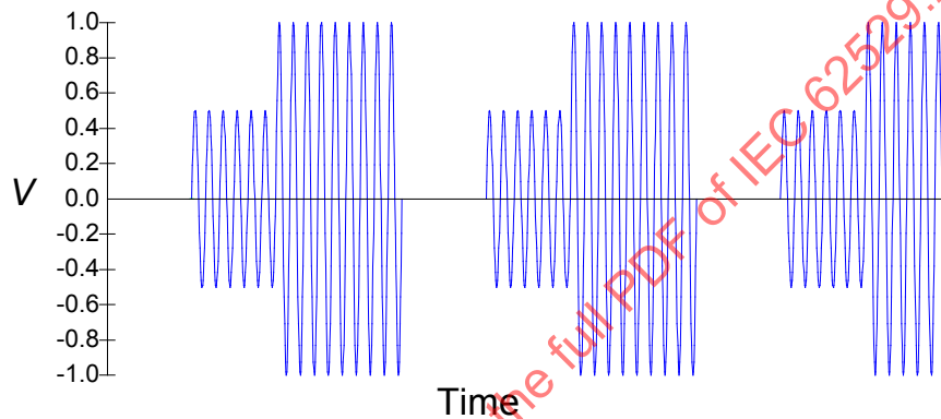
Figure B.32—PulseTrain
