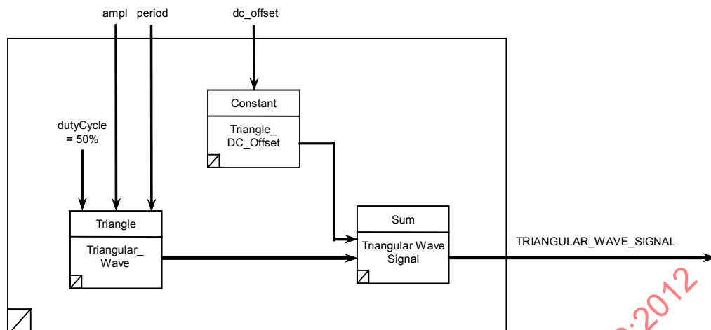
Figure E.59—TSF TRIANGULAR_WAVE_SIGNAL
