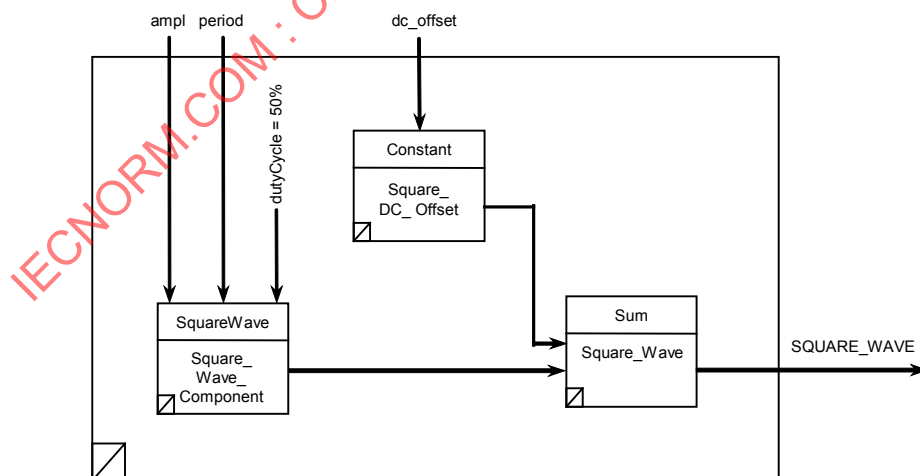
Figure E.45—TSF SQUARE_WAVE
