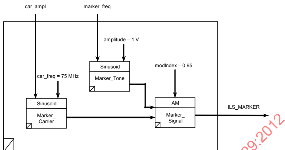
Figure E.23—TSF ILS_MARKER
