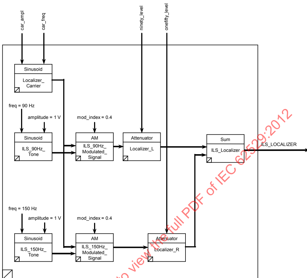
Figure E.21—TSF ILS_LOCALIZER
