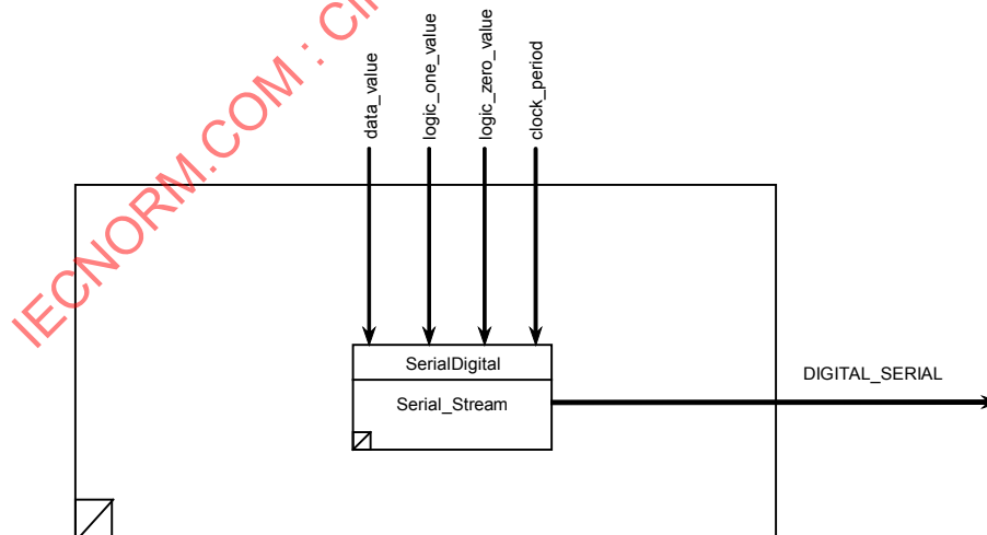
Figure E.9—TSF DIGITAL_SERIAL
