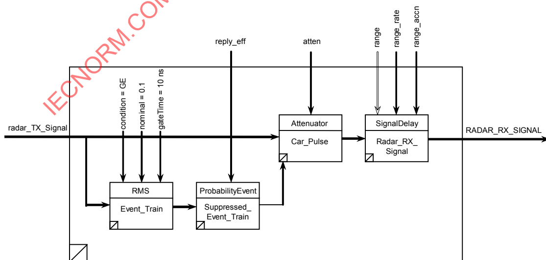
Figure E.35—TSF RADAR_RX_SIGNAL
