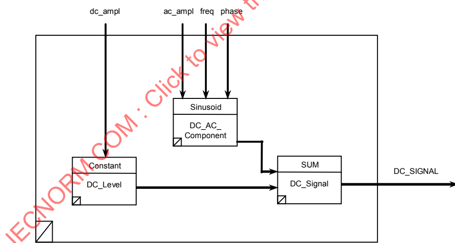
Figure E.5—TSF DC_SIGNAL
