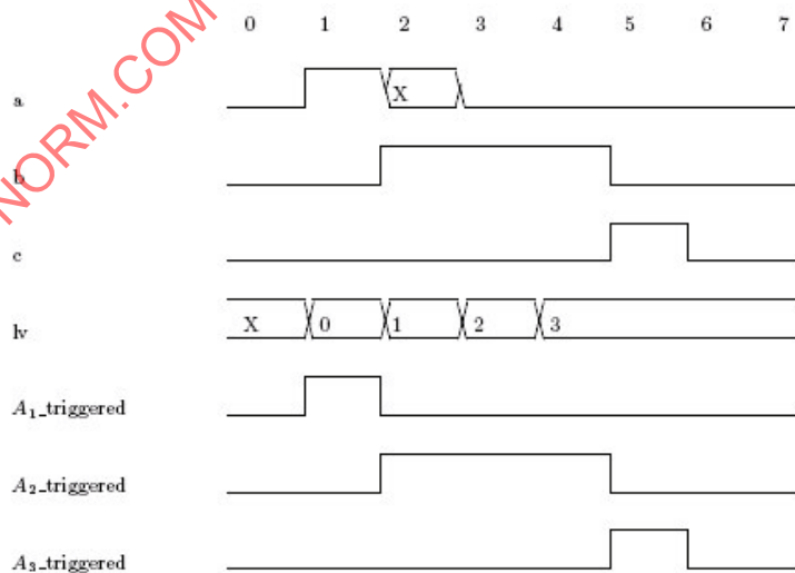
Figure 8—Match 1 of the SERE of Example 9
